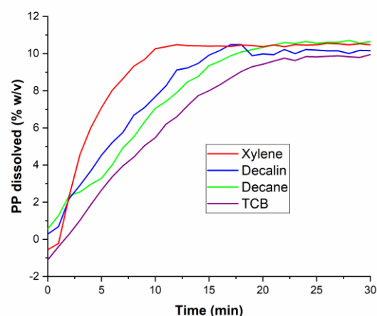
Fig. 6 Prediction of the dissolved polymer content in the different solvents by Raman spectroscopy (runs from 1 to 4 at 130°C with an agitation of 200 rpm).
