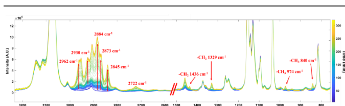
Fig. 1 Bands assignment of the raw Raman spectra of PP in TCB at 130^\circ\text{C} (Run 3) in the 700 - 1500\text{ cm}^{-1} and 2500 - 3200\text{ cm}^{-1} regions.
