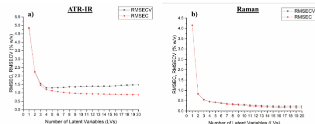
Fig. 3 Root Mean Square Error of Calibration and Cross-Validation according to the number of latent variables using the PLS model of the concentration of PP in TCB in a) ATR-IR and b) Raman.
