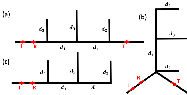
FIG. 1. (a) Schematic of a symmetric triple-stub cavity composed of a stub of length d_3 inserted between two stubs of length d_2 and separated by a segment of length d_1 . (b) The symmetric cavity is attached vertically to two ports from one side. (c) The symmetric cavity is attached only to one port from one side. I, R, and T denote the incident, reflected, and transmitted waves, respectively.
