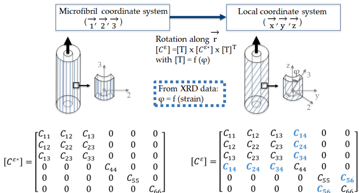
Fig. 6. Principle of the FE model taking into account the MFA and related stiffness matrix.
