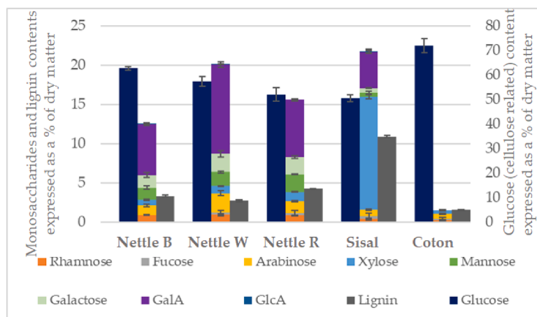
Fig. 4. Analysis of lignin, glucose (related to cellulose) and non-glucosidic monosaccharide content of nettle, sisal and cotton fibres used in this study.
