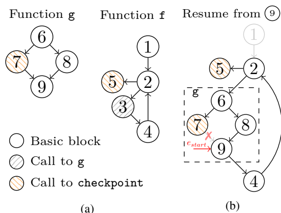
Fig. 6: Control flow graph of two functions f and g , where f calls g in basic block 3 (a). The analysis when resuming execution from basic block 9 is displayed in (b).
