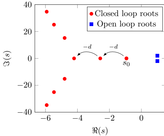
Fig. 1. Spectrum distribution of the characteristic function (4) corresponding to the closed-loop system of a second order unstable plant with a delayed proportional-derivative controller.
