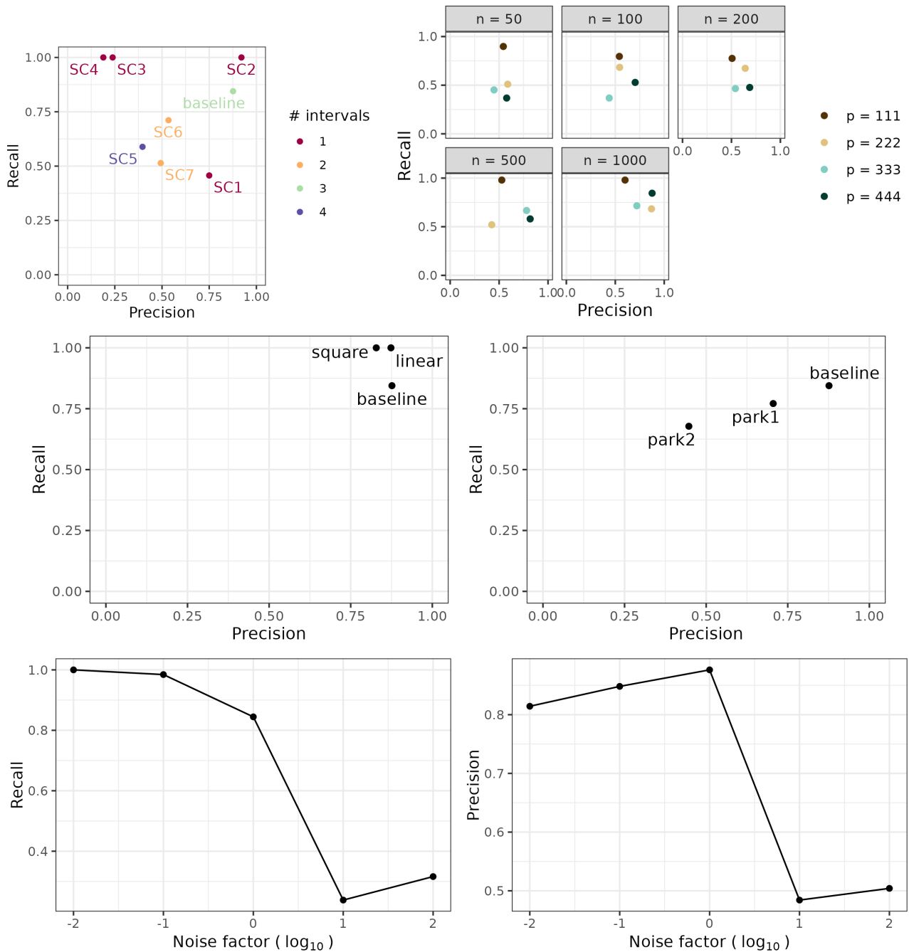
FIGURE 6 Impact of different variations of the simulation setting on the precision and recall of the method: (from left to right and top to bottom) number and size of intervals; n and p ; shape of the link function; shape of \beta ; signal-to-noise ratio.
