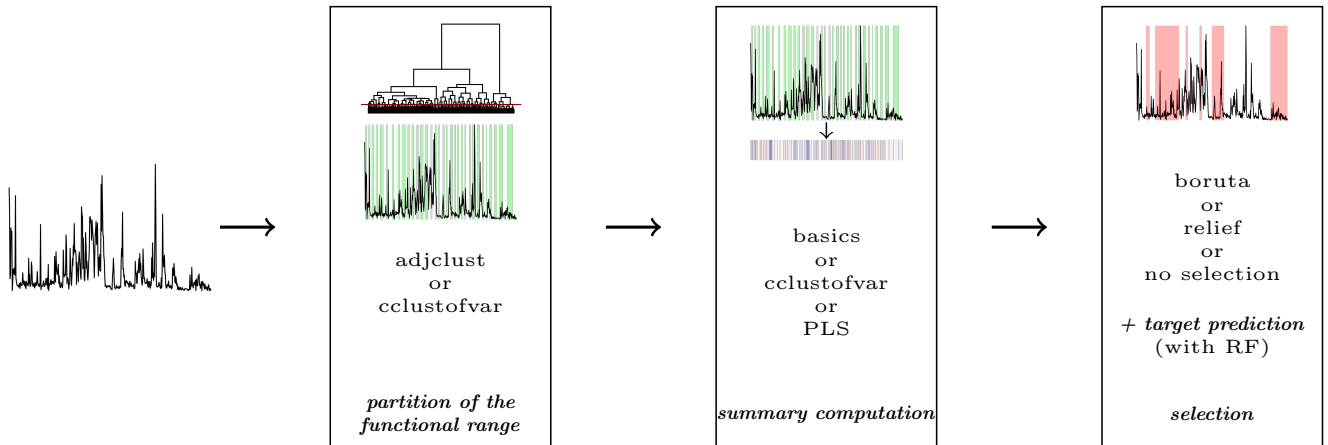
FIGURE 1 Overview of the different steps and variants of SFCB.
