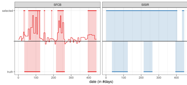
FIGURE 3 True (bottom) versus selected (top) intervals obtained by SFCB (left, red) and SISIR (right, blue) on the simulated dataset. The curve in the SFCB panel corresponds to the variable importance for the SFCB method with no variable selection (but the same choice for the groups and the summaries).
