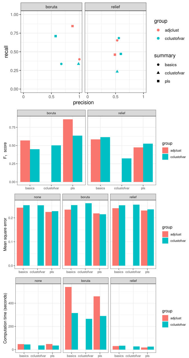
FIGURE 5 Precision & recall (first row), F_1 score (second row), mean square error (third row) and computational time (fourth row) obtained by the different variants of SFCB on the simulated dataset.
