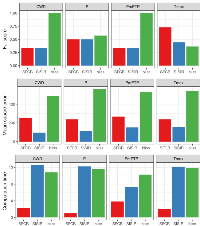
FIGURE 4 Quality criteria ( F_1 score, mean square error, and computation time) obtained by SFCB (red, left) and SISIR (blue, middle), and bliss (green, right) on the simulated dataset.
