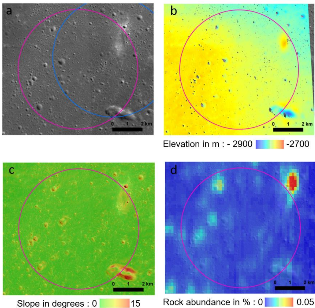
Figure 5: Close-up of the selected landing ellipse (SI-1) in Sinus Iridum. a) NAC imagery from image pair M1099022524 L + R. The ellipse from the Kaguya TC slope analysis is outlined in blue, whereas the location of the final landing ellipse, after analyses and refinements at the NAC scale, is outlined in magenta. b) Topography from the Sfs-based NAC DTM. c) Derived
