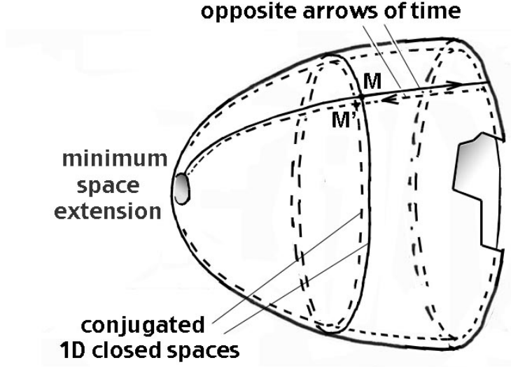
FIG. 4. , Didactic 2D image of the Janus Cosmological Model
