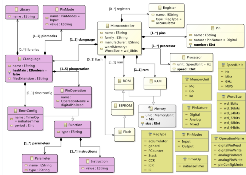
Figure 5. Microcontroller metamodel 4.2. Transformation step for code generation
