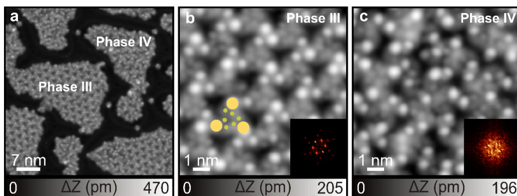
Figure S8. Phase transformation of 5-F self-assembled structures by annealing at 100 °C on Au(111). (a) Large-scale STM image of the new phases. (b, c) Close-up views of phase III and phase IV, respectively. Insets show corresponding 2D-FFT images. Scanning parameter: V = 0.2 V and I = 10 pA.
