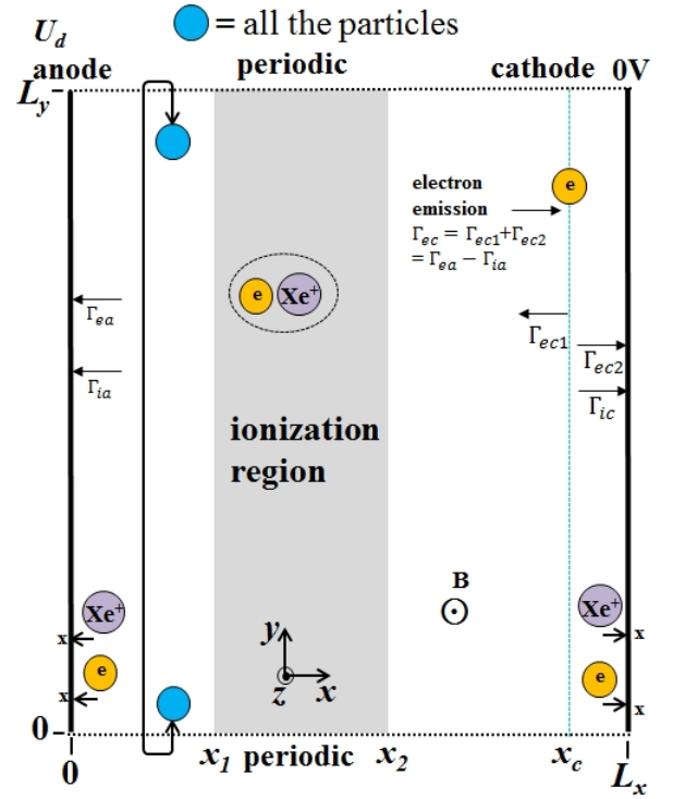
FIG. 7. Computational domain. The parameters x_1 , x_2 , and x_c refer to left and right injection planes and the axial position of the cathode. The charged particle fluxes averaged along the y direction \Gamma_{ea} , \Gamma_{ia} , \Gamma_{ec} , \Gamma_{ec1} , \Gamma_{ec2} , and \Gamma_{ic} stands for electron and ion fluxes at the anode, through the cathode, and through the exhaust planes, respectively.
