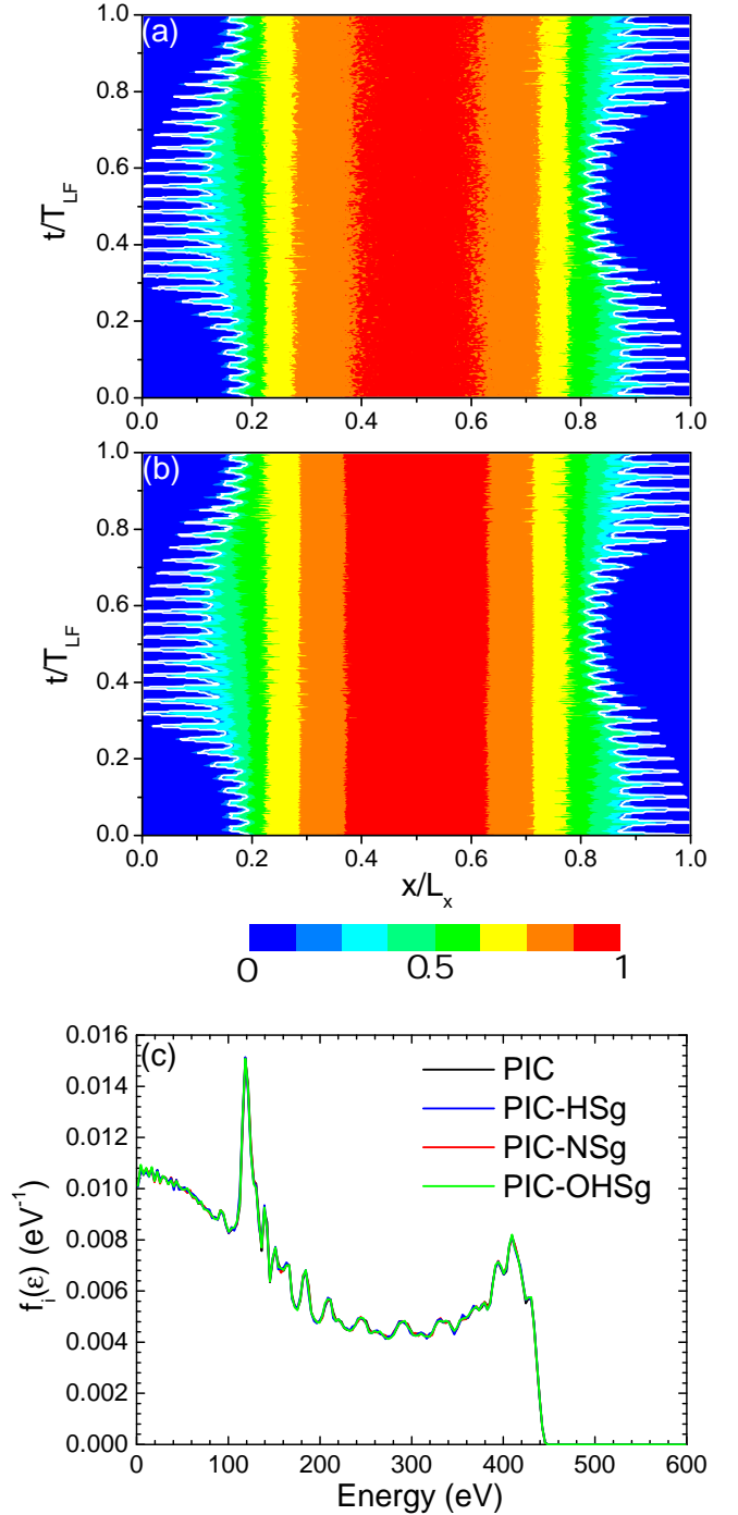
FIG. 7. CASE B. Axial and time (one LF cycle reconstructed after averaging over 60 LF cycles results after convergence) profiles of the ionization source term and sheath edge for (a) PIC and (b) PIC-NSg algorithms, (c) Time averaged ion energy probability function at the RF electrode normalized such that \int_0^\infty f_i(\epsilon) d\epsilon = 1 . The maximum of the ionization source term is 3.4 \times 10^{20} \text{ m}^{-3} \text{ s}^{-1} . Standard PIC results correspond to 256^2 grid nodes. Sparse PIC results correspond to n = 8 , the results of the offset method corresponds to l^0 = 3 , and l^1 = 1 .
