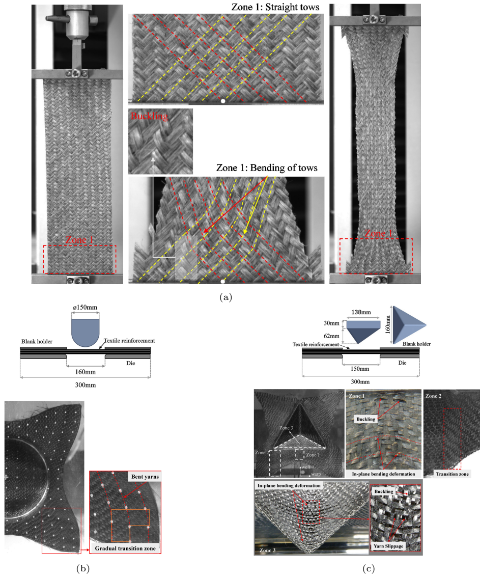
Figure 1: In-plane bending deformations of textile reinforcement. (a) Bias-extension test of Twill Flax. (b) Four layers G1151 hemisphere forming. (c) Two layers G1151 tetrahedron forming.
