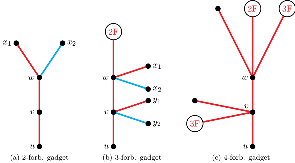
Figure 3: Examples of forbidding gadgets. “ kF ” inside a node indicates a k -forbidding gadget is attached at some vertex. Edges in red and blue form a h.i. 2-edge-colouring omitting conflicts along uv (root edge).
