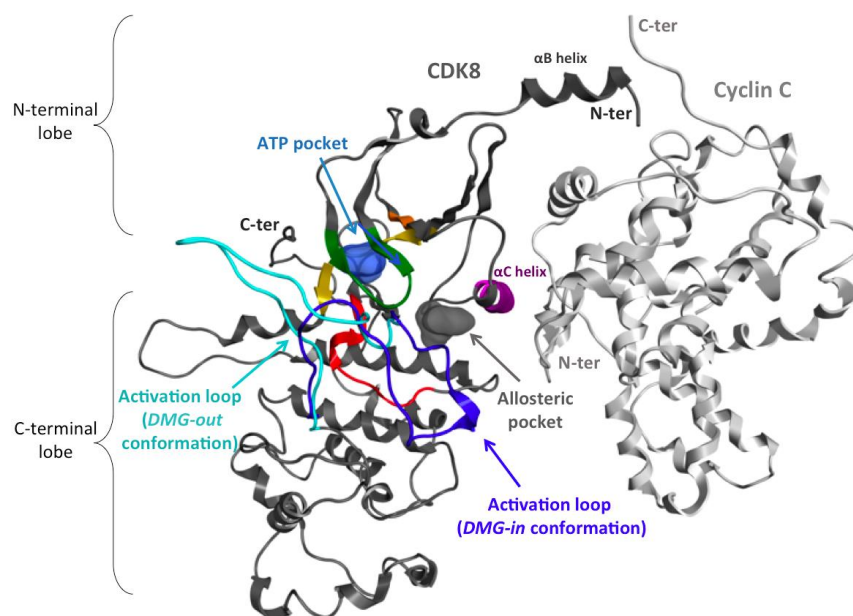
Figure 8. Ribbon representation of the CDK8–CycC complex. Cyclin C (CycC, PDB ID: 4F6U) is colored in light grey and CDK8 in dark gray, except the conserved motifs of the kinase domain. Among these motifs, the activation loop in the DMG-out conformation (inactive form) is colored in cyan (PDB ID: 4F6U), and that in the DMG-in conformation (active form) is dark blue (PDB ID: 4F7S).
