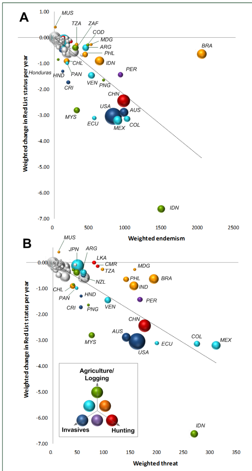
Figure S5. Relationship between each country's responsibility to conservation and its contribution to changes in the global conservation status of birds, mammals and amphibians. Responsibility measured by: (A) weighted endemism; (B) weighted threat. Dashed lines are the regression lines fitted through the origin: (A) R^2 = 0.57 ; (B) R^2 = 0.70 ( n=195 ; p<0.001 ). Circle size is proportional to each country's Gross Domestic Product in 2009. Circle color indicates the main threat (or combination of threats) for selected countries. See Table S2 for country codes.
