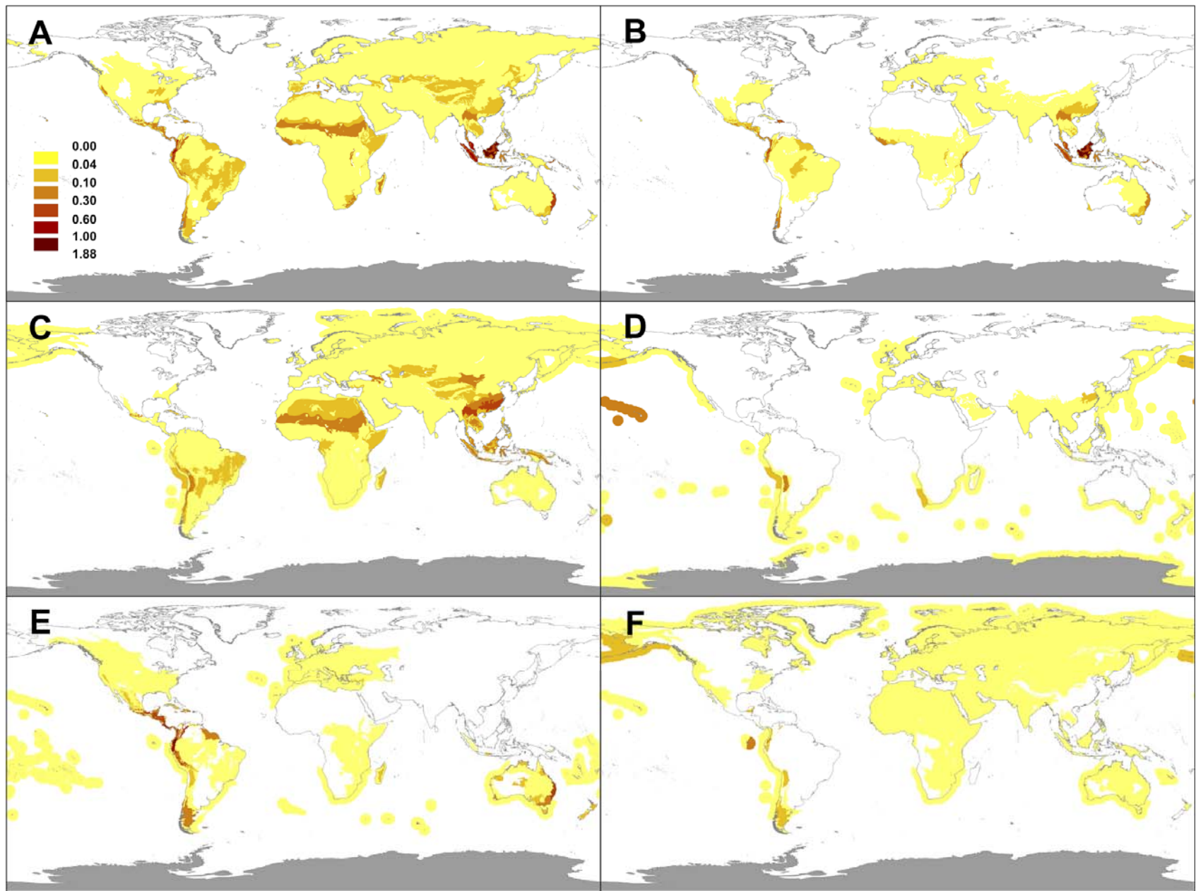
Figure S4. Weighted impact of each threat to the deterioration in global species conservation status, across ecoregions: (A) agriculture; (B) logging; (C) hunting and trapping; (D) fisheries; (E) invasives; and (F) climate change. The same color scale is used across panels, hence shades are directly comparable.
