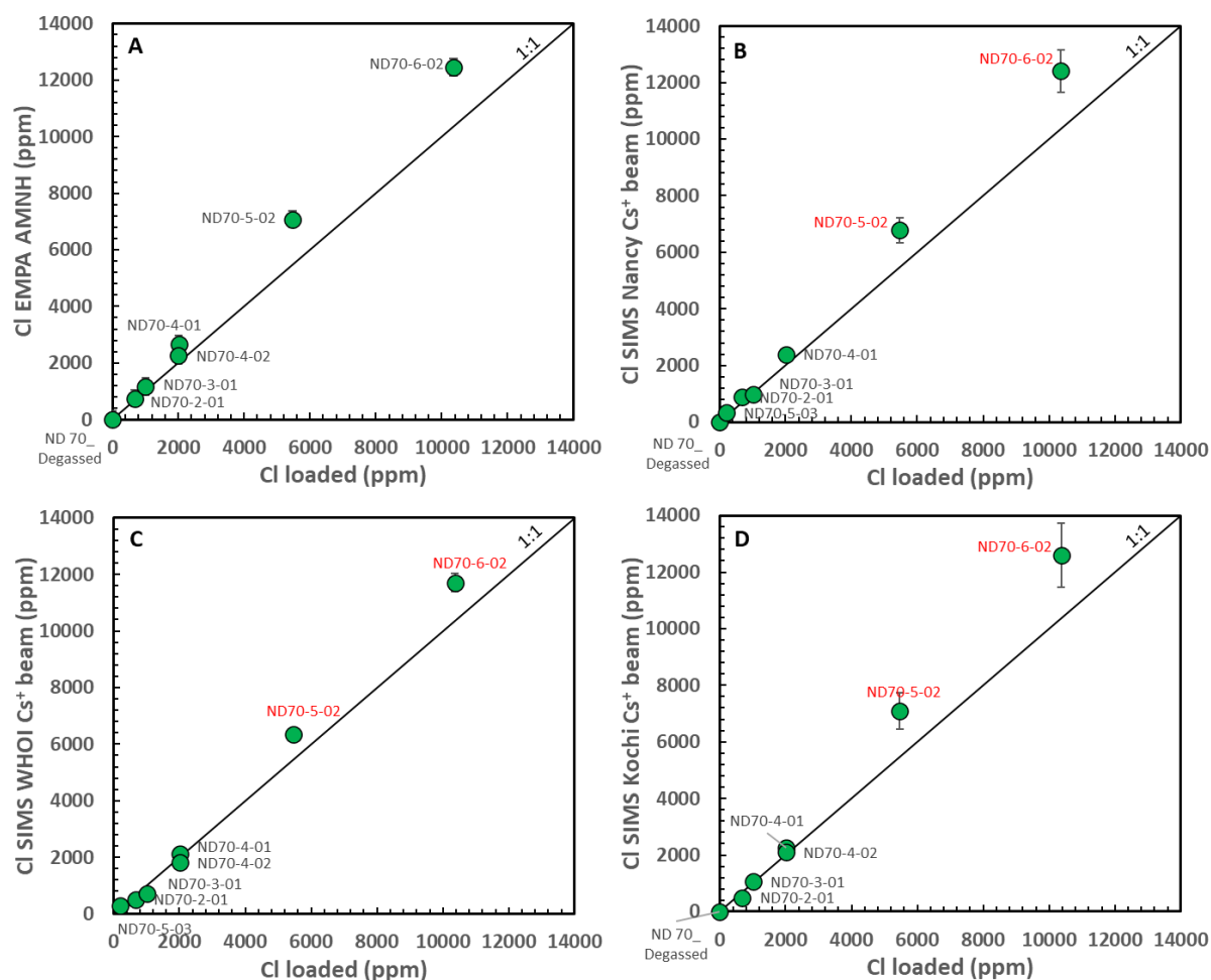
Figure 4: Comparison between the expected (i.e., loaded) and measured Cl content in the new reference materials. Samples labelled in red were measured outside their respective calibration ranges (Fig. S5).
