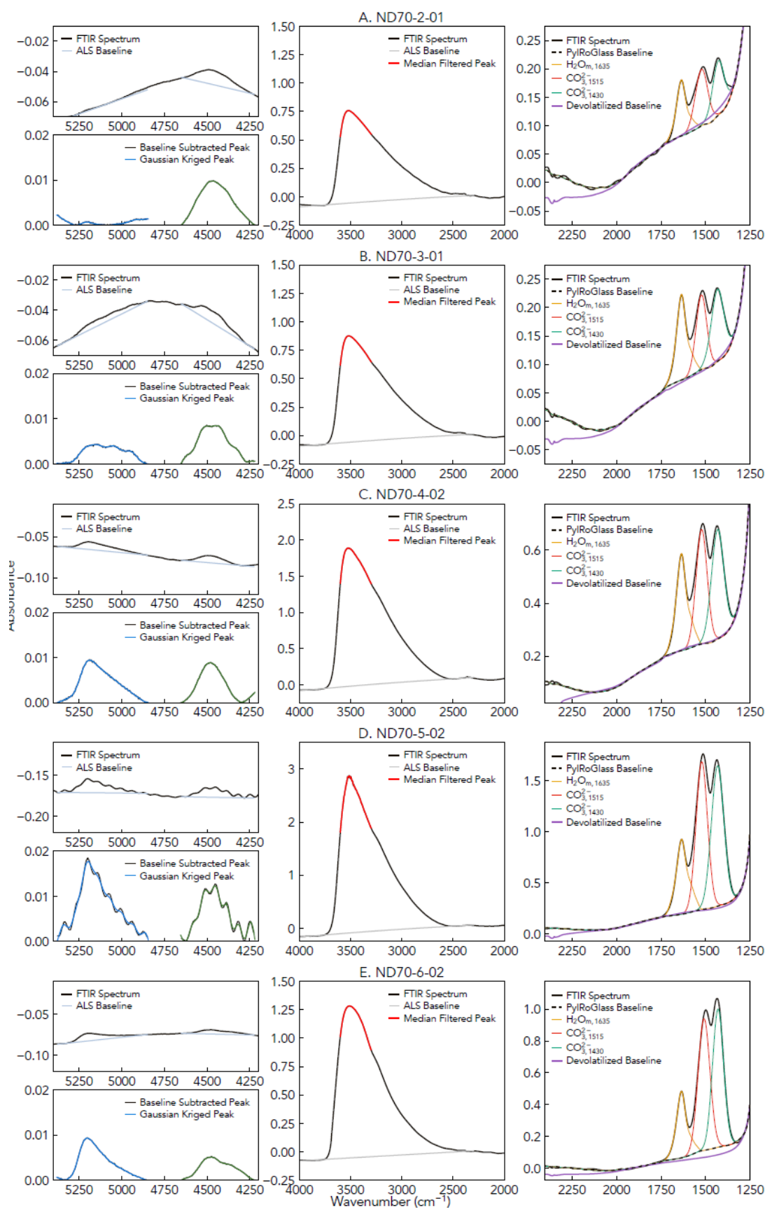
Figure S9: FTIR spectra of ND70 series glasses and spectra fitting with the PyIRoGlass software (Shi et al., 2023).
