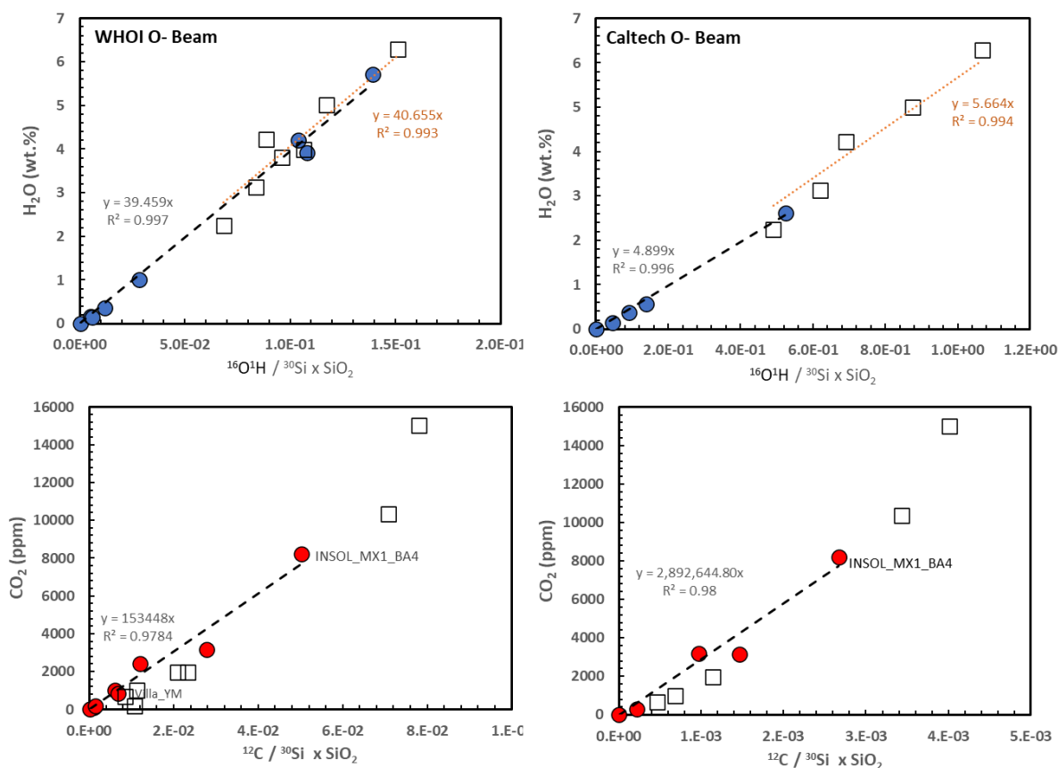
Figure S7: Signal retrieved by SIMS using a \text{O}^- primary beam at WHOI and Caltech Ion Probe facilities. Filled circle symbols show glasses used as standards for volatile analyses (marked as “Other glasses analysed” in Table 5) in addition to INSOL_MX1_BA and VILLA_YM whose volatile contents were determined as part of this study. Square symbols represent the new ND70 reference series plotted on the y-axes according to their expected (i.e., loaded) values. Data in Tables S6 and S7. Black dashed lines are the calibration lines while red dotted lines are linear regressions through the ND series glasses.
