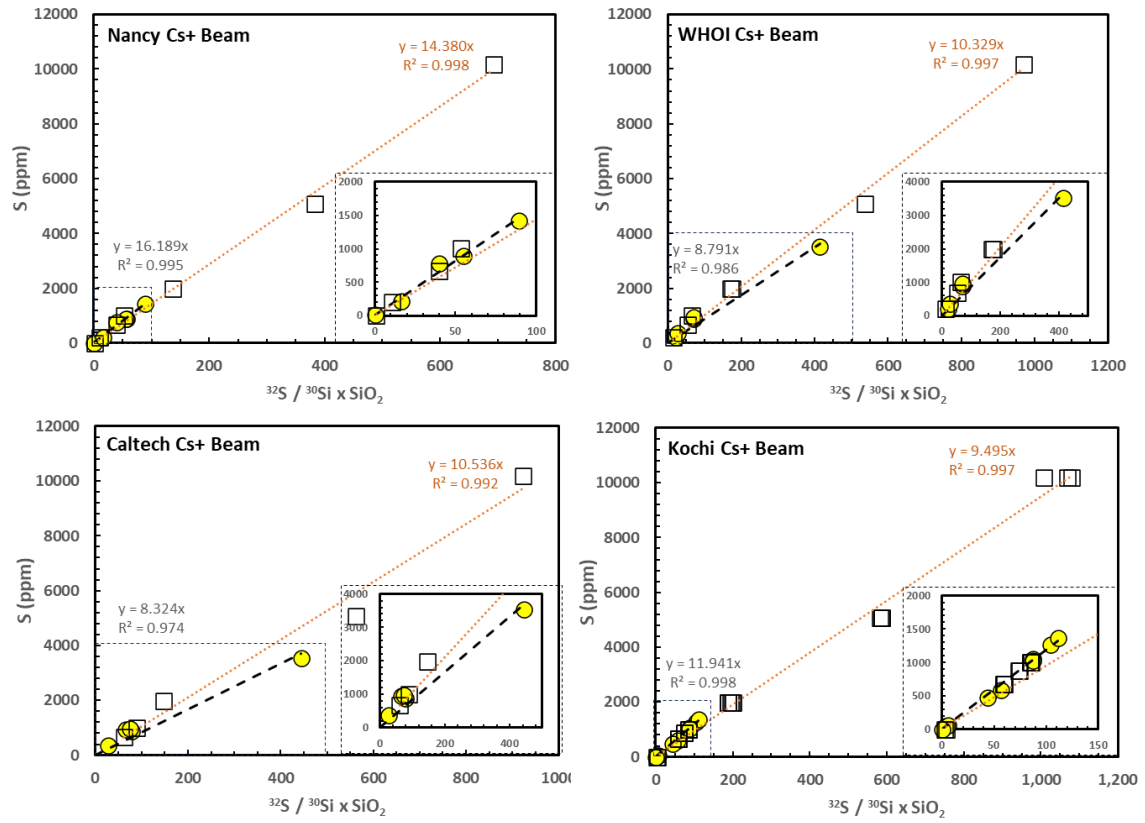
Figure S4: Same as Fig. S2, for ^{32}\text{S} .
