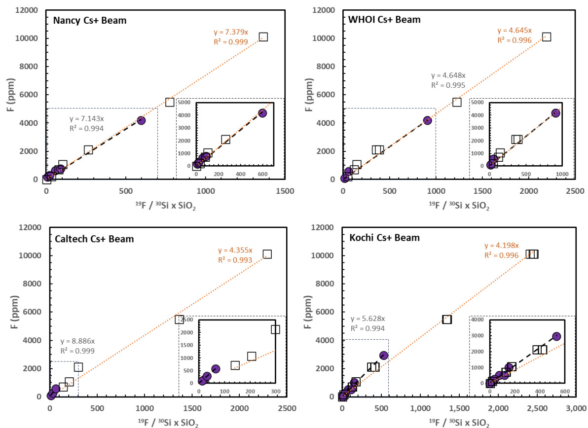
Figure S6: Same as Fig. S2, for ^{19}\text{F} .
