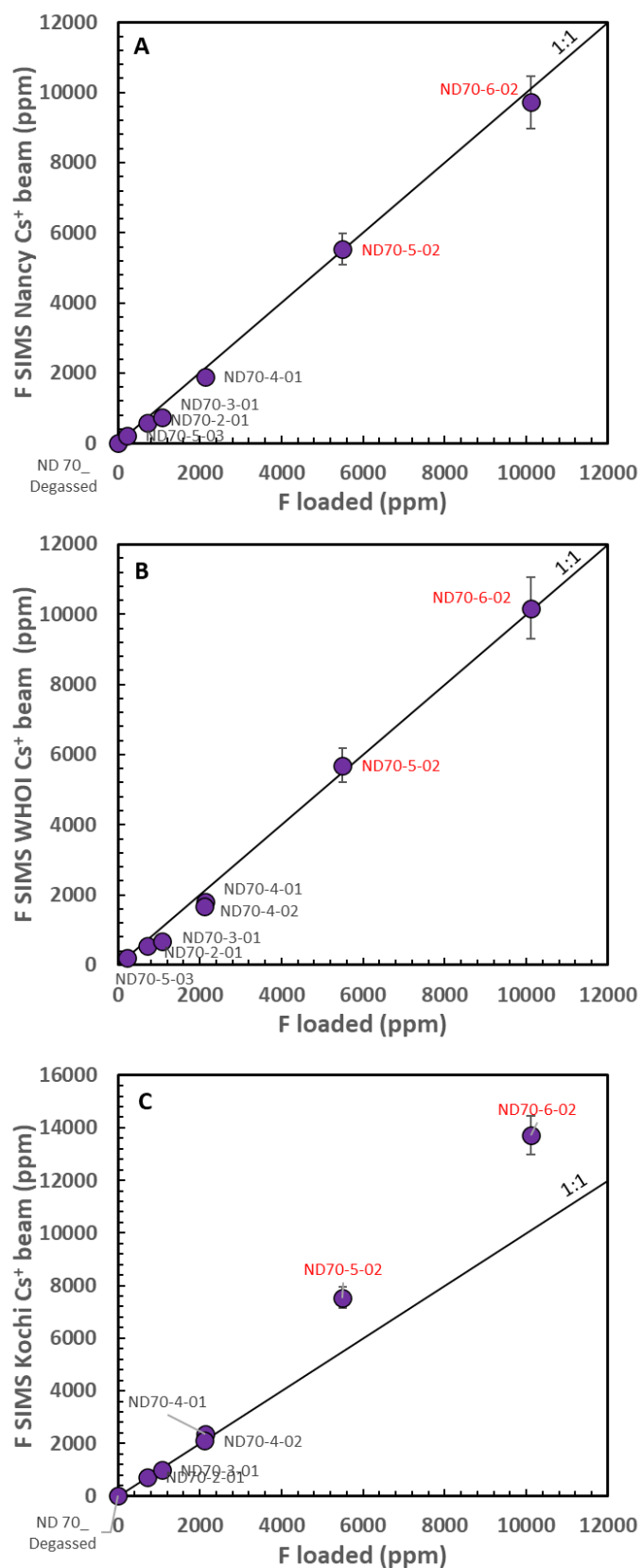
Figure 5: Comparison between the expected (i.e., loaded) and measured F content in the new reference materials. Samples labelled in red were measured outside their respective calibration ranges (Fig. S6).
