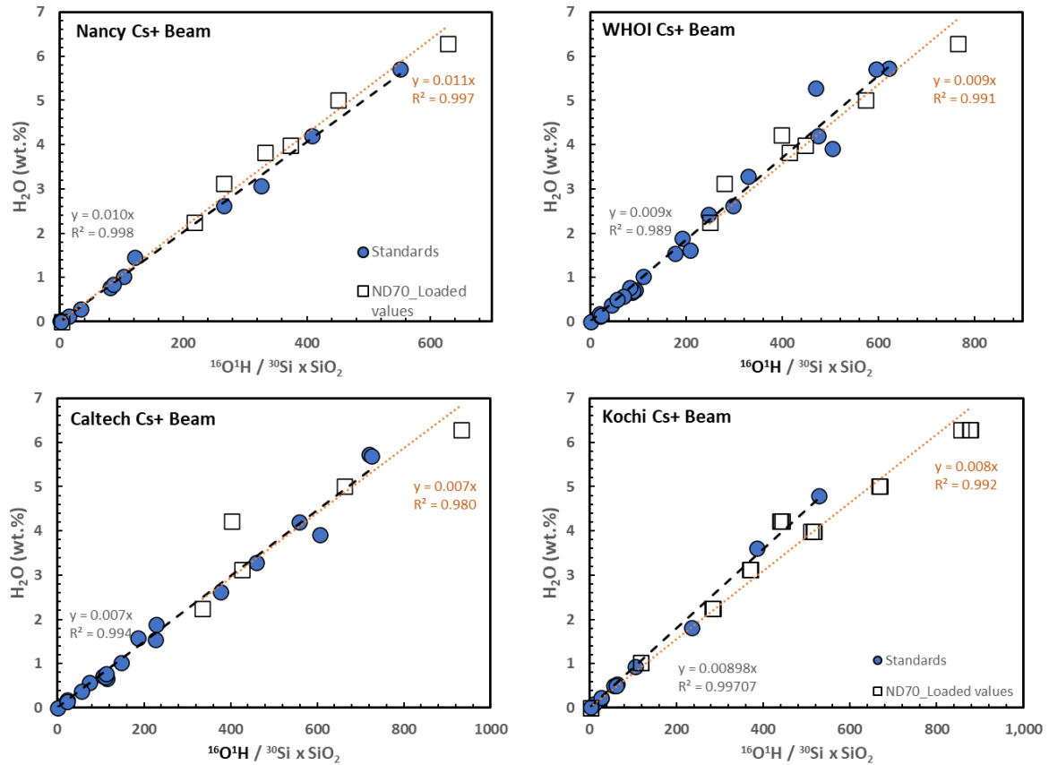
Figure S2: ^{16}O^1H signal retrieved by SIMS using a Cs^+ primary beam at Nancy, Kochi, WHOI and Caltech Ion Probe facilities. Filled circle symbols show glasses used as standards for volatile analyses (marked as “Other glasses analysed” in Table 5) in addition to INSOL_MX1_BA and VILLA_YM whose volatile contents were determined as part of this study. Square symbols represent the new ND70 reference series plotted on the y-axes according to their expected (i.e., loaded) values. Data in Tables S3 to S5. Black dashed lines are the calibration lines while red dotted lines are linear regressions through the ND series glasses.
