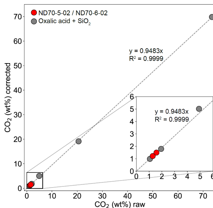
944 945 Figure S1: Elemental Analyser secondary calibration. CO 2 (wt%) raw indicates the raw EA 946 result calibrated by acetanilide. CO 2 (wt%) corrected is calibrated by a series of oxalic acid 947 and SiO 2 mixtures. Gray circles are oxalic acid and SiO 2 mixtures. Red circles are 948 ND70_5_02 and ND70_6_02. Dashed line is the calibration line based on oxalic acid and 949 SiO 2 . 950
