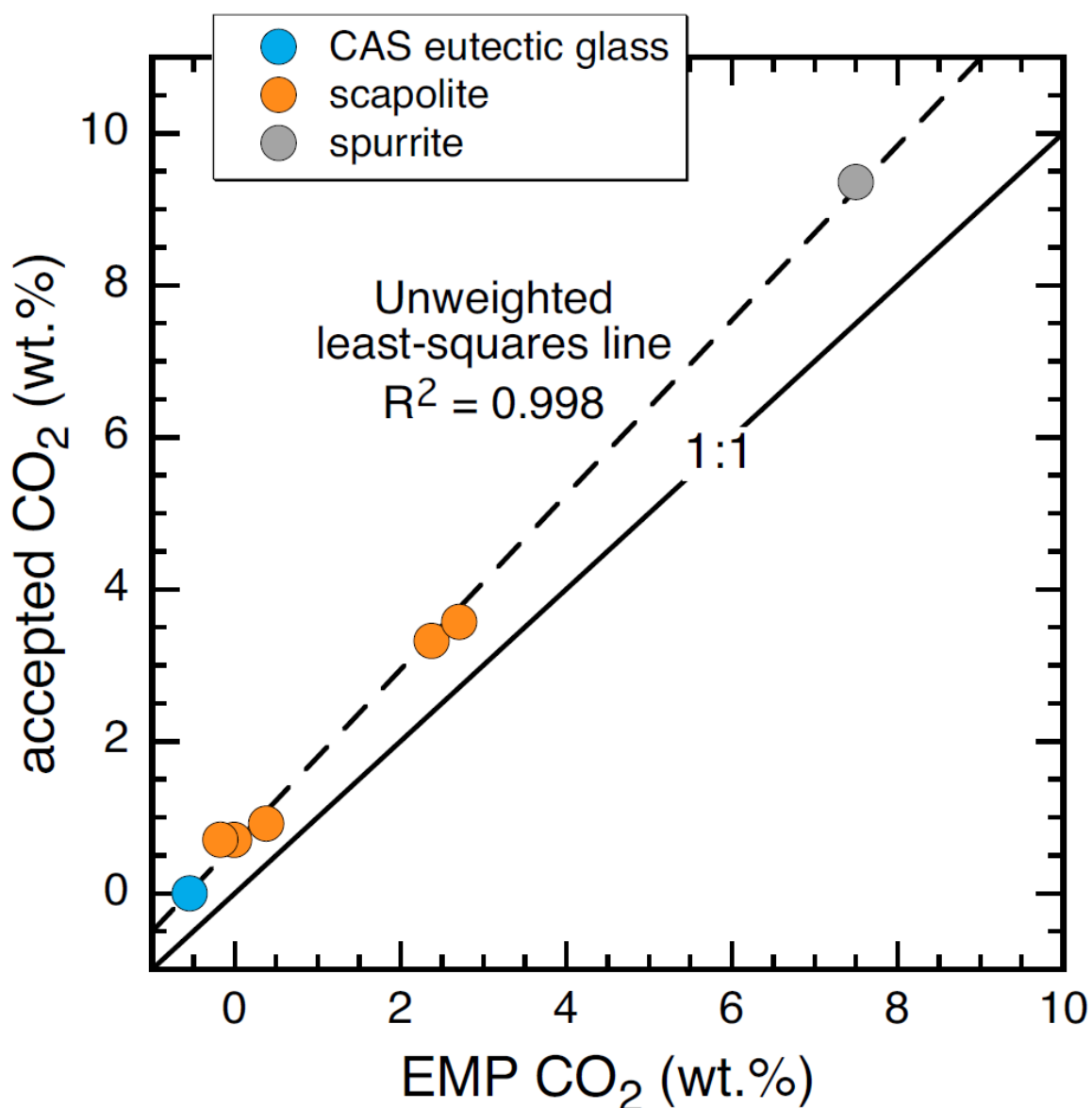
Figure S8: Electron microprobe CO 2 contents vs. accepted CO 2 contents (all in wt.%) for the secondary standards. The CaO-Al 2 O 3 -SiO 2 eutectic is bounded by the pseudowollastonite, anorthite, and tridymite liquidus fields; the glass was fused at 1-atm in air and is assumed to have a CO 2 content of zero. Scapolite CO 2 contents determined by NRA; the CO 2 content of the spurrite is based on mineral stoichiometry. The dashed line is an unweighted least-squares fit to the seven secondary standards.
