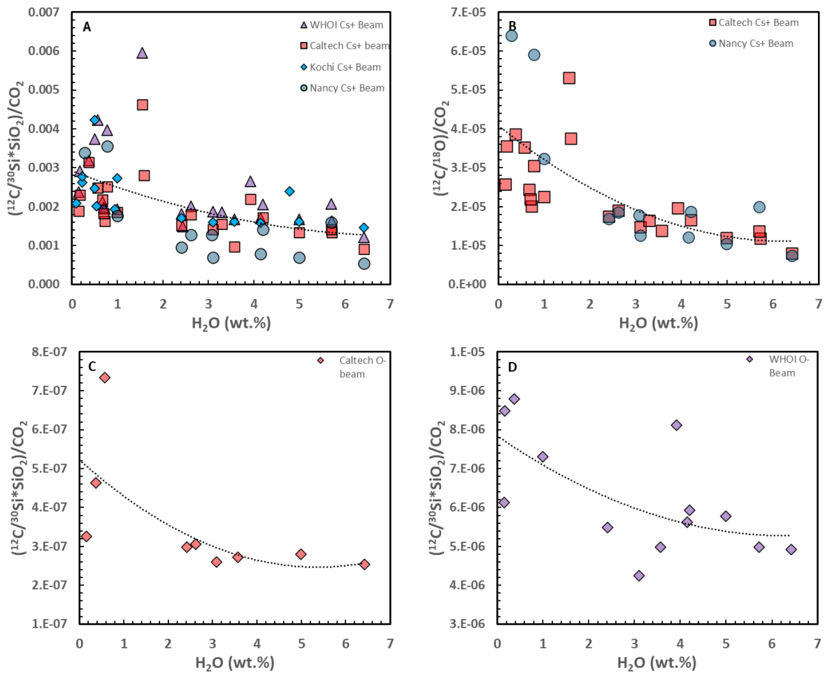
Figure 8: Effect of water on the ((^{12}\text{C}/^{30}\text{Si}) \times \text{SiO}_2)/\text{CO}_2 and (^{12}\text{C}/^{18}\text{O})/\text{CO}_2 ratios measured by SIMS (i.e., the calibration line). The results of four SIMS sessions using a Cs + primary beam and two SIMS sessions using a O - primary beam are reported. In all cases the glass water content seems to greatly reduce the ionization efficiency of 12 C. Data used to generate the figure are reported in Table S9. Dotted lines are 2 nd order polynomial best fit to all data.
