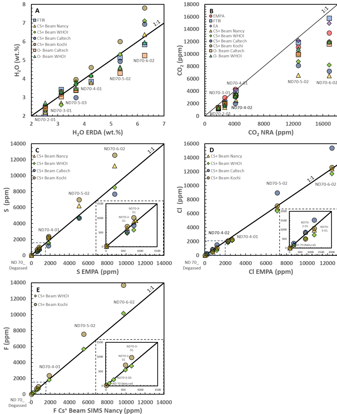
Figure 7: Comparison of measured H_2O , CO_2 , S , Cl and F volatile content in ND70-series glasses by several techniques. With the exception of the last panel, the X-axis of each plot is the technique we have highest confidence in. All F analyses (panel E) were done by SIMS. Y-axis gives the value measured by all other techniques.
