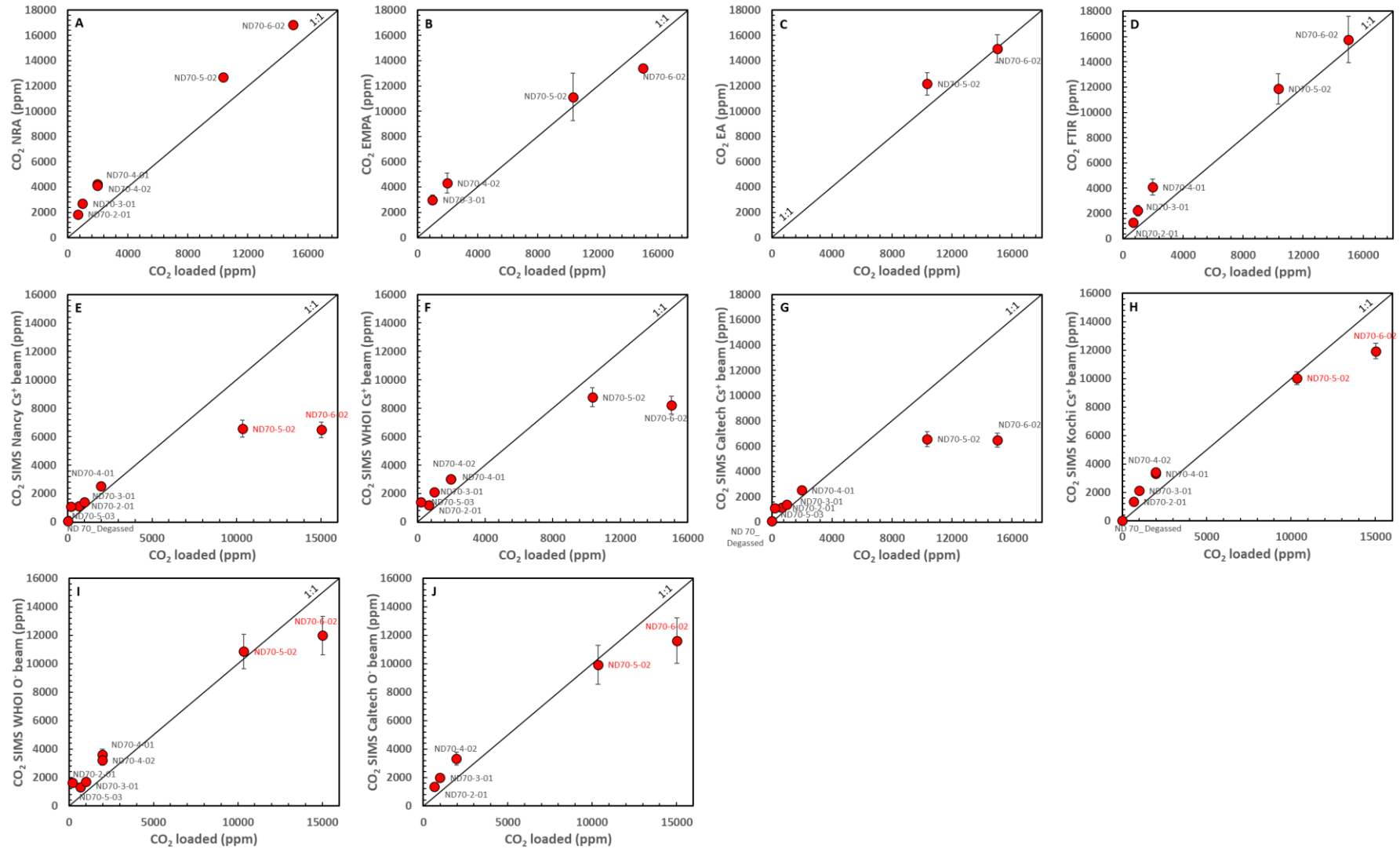
Figure 2: Comparison between the expected (i.e., loaded) and measured CO 2 content in the new reference materials. Samples labelled in red were measured outside their respective calibration ranges (Fig. S3 and S7).
