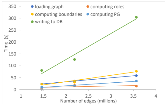
Figure 6: Data processing times on RDF datasets.
