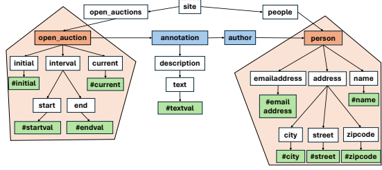
Figure 2: Collection graph obtained from xmark.xml (Fig. 1).
