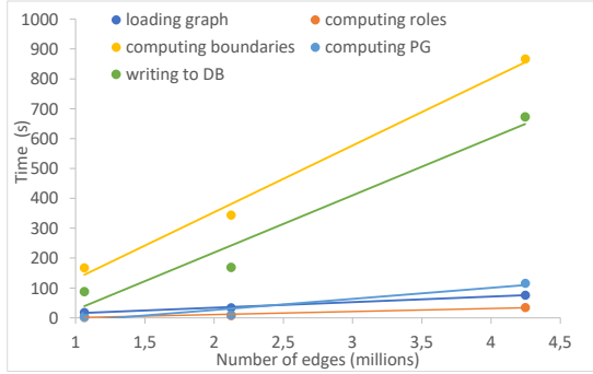
Figure 5: Data processing times on XML datasets.
