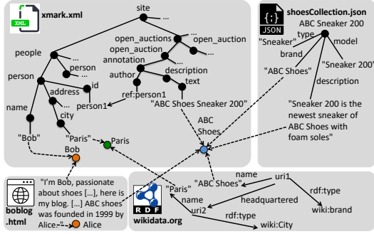
Figure 1: A ConnectionLens graph built from 4 datasets
