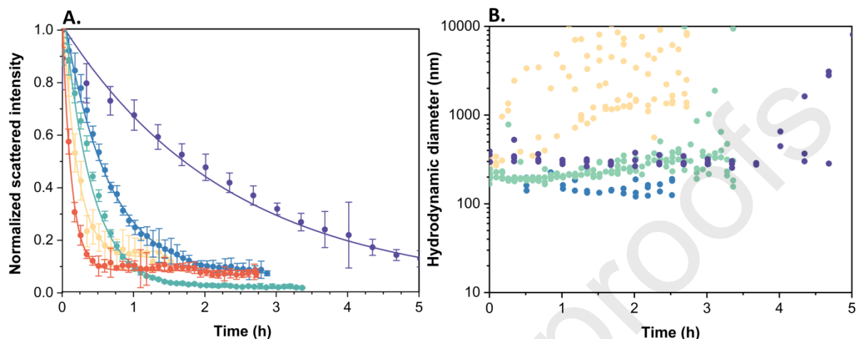
Figure 7. A. Scattered intensities measured as a function of incubation time with first-order exponential decay fit for a concentration of 0.1 \text{ mg}\cdot\text{mL}^{-1} at 37^\circ\text{C} ; B. Evolution of the DLS diameter obtained with the cumulant fit. (blue) pure water; (yellow) PBS 1\times ; (green) PBS 0.1\times ; (orange) NaCl 137 \text{ mM} ; (purple) \text{H}_2\text{O}/\text{EtOH} 85/15 \% v:v.
