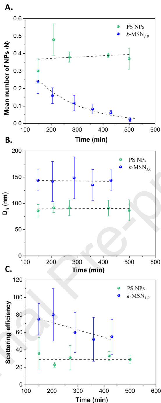
Figure 8. Confocal DLS dissolution studies on k -MSN 1,0 using a concentration of 0.1 mg·mL -1 at 37°C (blue) and on PS reference particles (green). A. The average number of NPs \langle N \rangle in the confocal volume, B. Mean hydrodynamic diameter, D_h , and C. Scattering efficiency per NP. The error bars correspond to the limit values obtained when repeating the measurements under the same conditions.
