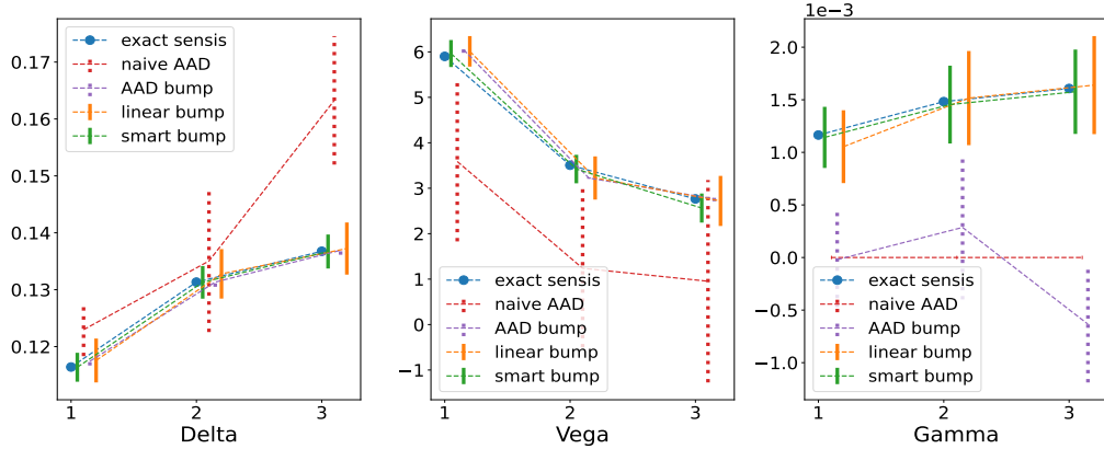
(a) d = 3 and m = 10^5 paths.
