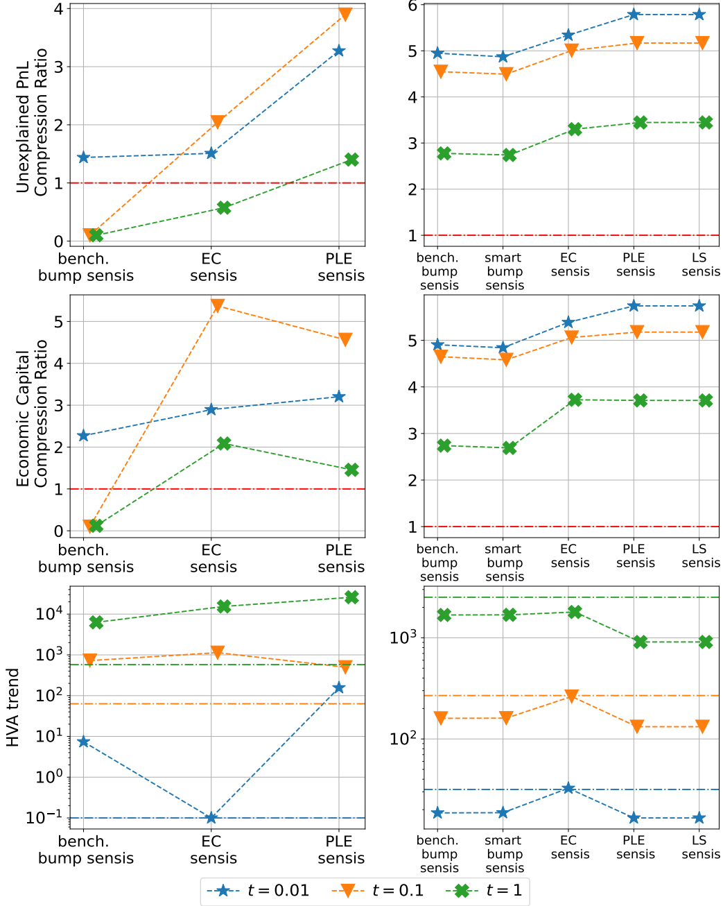
Figure 4: Compression ratios of UPL ( top ), EC ( middle ), and HVA trends c ( bottom ), for various \delta\text{CVA}_t^\theta + \text{LGD}_t hedging approaches in Section 5.1 ( left ), and \delta\text{CVA}_t^\theta hedging approaches in Section 6.1 ( right ). Horizontal dash-dot lines correspond to the unhedged case with \Delta = 0 in (15) and (20).
