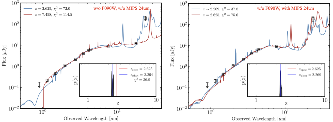
Fig. 3. NIR-to-MIR SED of COSBO-7 fitted with Bagpipes . Left: Fitting without the F090W upper limit and without 24 \mu\text{m} photometry with the PDF( z ) shown in the subpanel. We also show the SEDs and \chi^2 for both z = 2.625 and 7.458 cases. Right: Best fit with MIPS 24 \mu\text{m} photometry and without the F090W limit. We present the PDF( z ) with z_{\text{spec}} in the subpanel.
