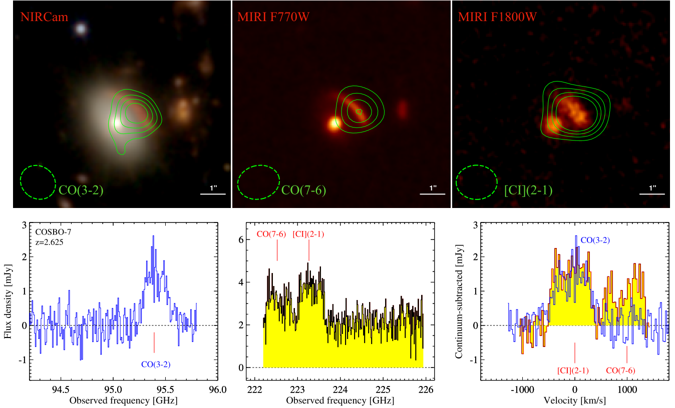
Fig. 1. JWST images and ALMA spectra of COSBO-7. Top: NIRCcam color image (Blue: F090W+F115W+F150W; Green: F200W+F277W; Red: F356W+F410M+F444W), and MIRI images overlaid with contours of CO and [CI] emission. Contours are shown at 4, 6, 8, and 10 \sigma levels. The beams are shown as dashed ellipses. Bottom: Left and middle panels show the CO(3–2) and CO(7–6)+[CI](2–1) spectra in observed frequencies. The right panel shows the continuum-subtracted spectra as a function of velocity.
