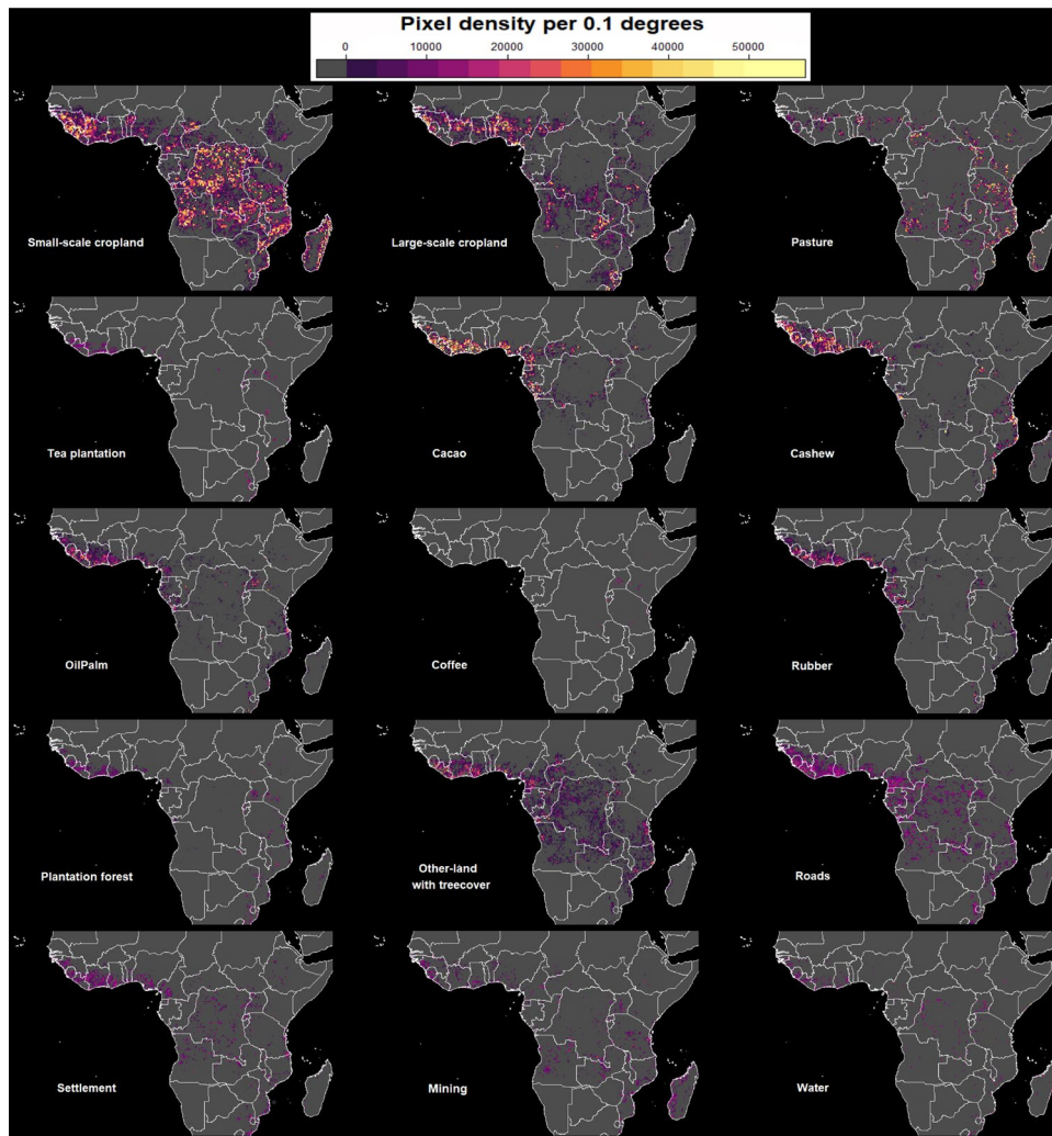
Figure 6. Hotspots of different land-use following deforestation in Africa along 30° south and 30° north, for the year 2001 to 2020. The colorbar shows the estimated pixel density of each land-use in a given location.
