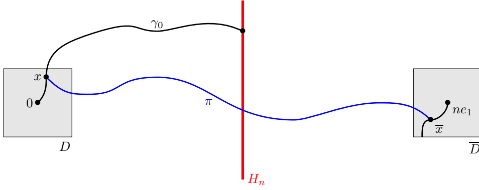
Figure 2: The path \pi is contained in the infinite cluster I and has controlled length.
