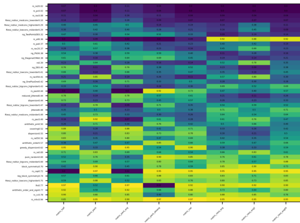
6 points, shape (32, 32, 4)
