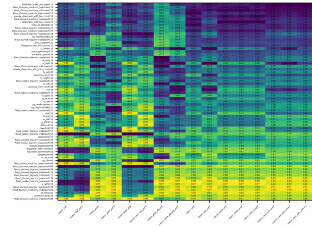
6 points, shape (16, 16, 2)
