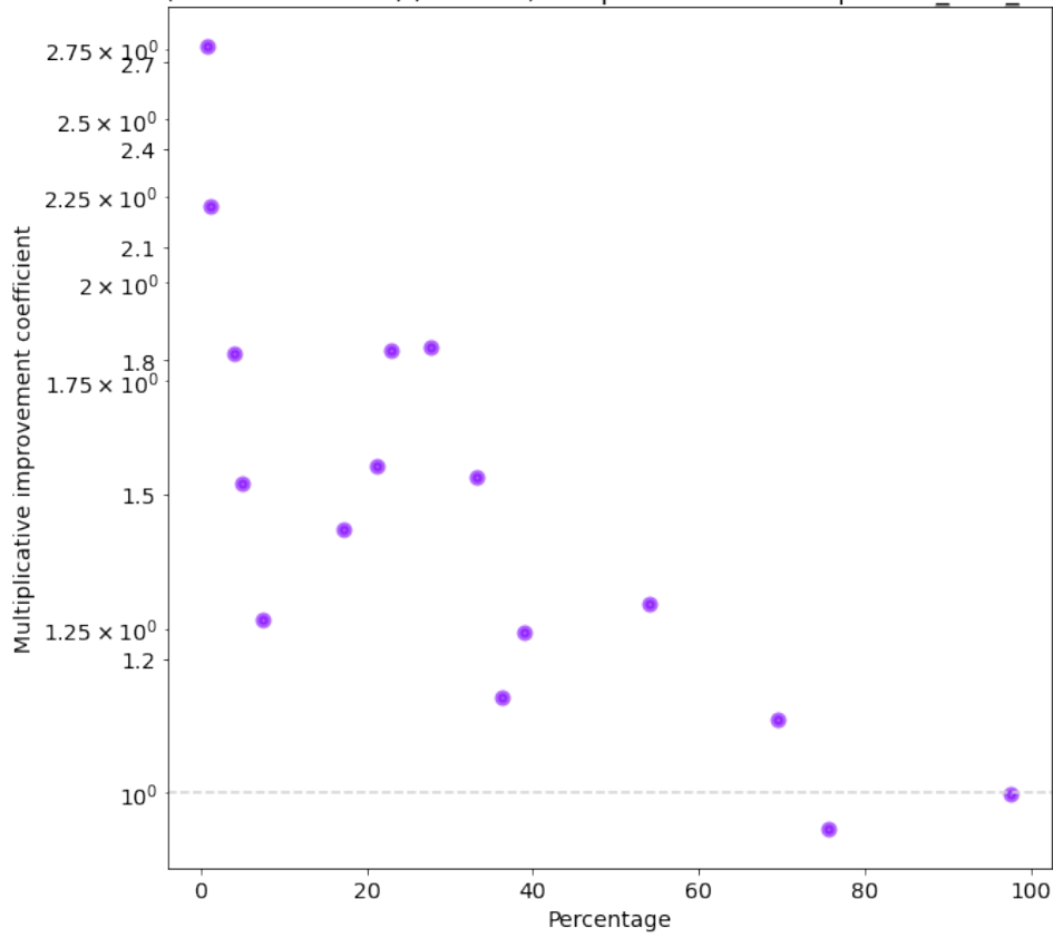
Figure 11. LDM1 with LS 64x64x4. Comparison of dispersion-with-conv and standard LDM1 (pure-random) for various prompts: the curves present the multiplicative percentage of batches containing images with at least 2 different dominant colors for the following parameters: K = 1.2 , batch size = 50. In general we get better improvements (greater y-axis values) for least represented groups (lower x-axis values).
