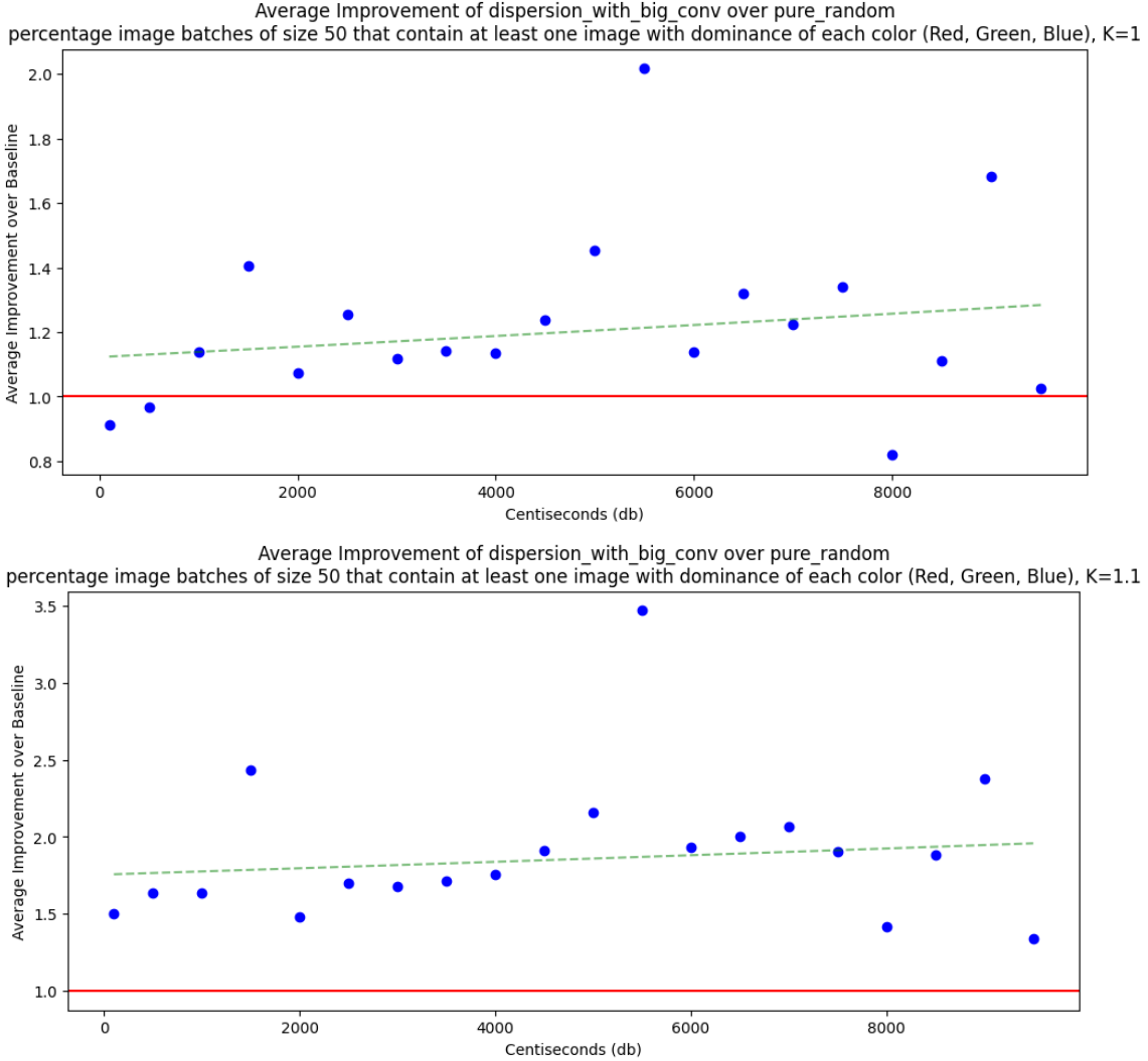
Figure 14. This figure illustrates the change in color diversity (LDM1 with LS 64x64x4) depending on the computational cost for the 'dispersion-with-big-conv' method. Similarly to the 'dispersion-with-conv' method, there is a noticeable improvement in the percentage of image batches with complete color representation compared to the 'pure-random' approach, increasing slightly with the computational budget.
