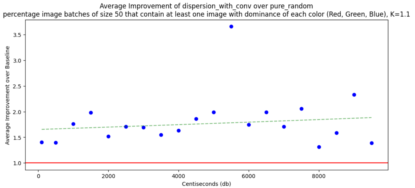
Figure 12. LDM1 with LS 64x64x4. This figure shows the variation in color diversity depending on the computational cost for the 'dispersion-with-conv' method. It compares the improvement in color diversity against the 'pure-random' baseline, demonstrating a slight increase in the percentage of image batches containing all dominant colors as the computational budgets progresses: we do not need a big computational power. In Section "Statistics in LDM3/ LDM2: LS 512x512x4", 3 seconds, we also show that 3s is enough for an impact on a larger LS 512x512x4 as the one of Large-LDM.
