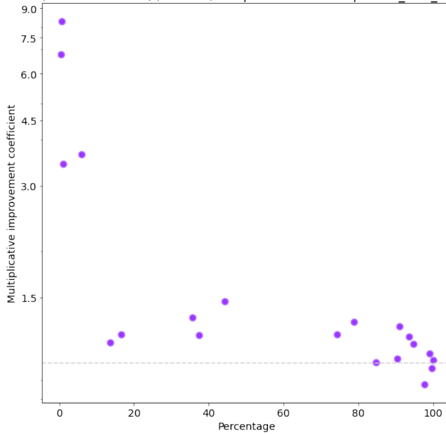
Figure 10. LDM1 with LS 64x64x4. Comparison of dispersion-with-conv and standard LDM1 (pure-random) for various prompts: the presented numbers are the multiplicative percentage of batches containing images with at least 2 of the 3 different dominant colors for the following parameters: K = 1.1 , batch size = 50. In general we get better improvements (greater y-axis values) for least represented groups (lower x-axis values).
