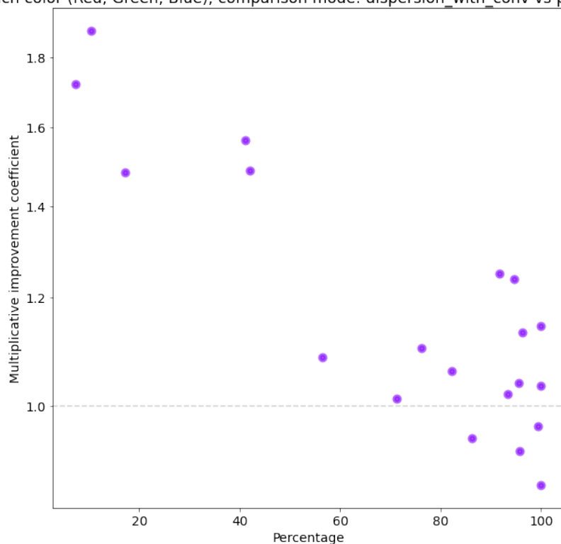
Figure 9. LDM1 with LS 64x64x4. Comparison of dispersion-with-conv and standard LDM1 (pure-random) for various prompts: the presented numbers are the multiplicative percentage of batches containing images with all 3 dominant colors for the following parameters: K = 1 , batch size = 50. In general we get better improvements (greater y-axis) for the most difficult cases (low x-axis value).
