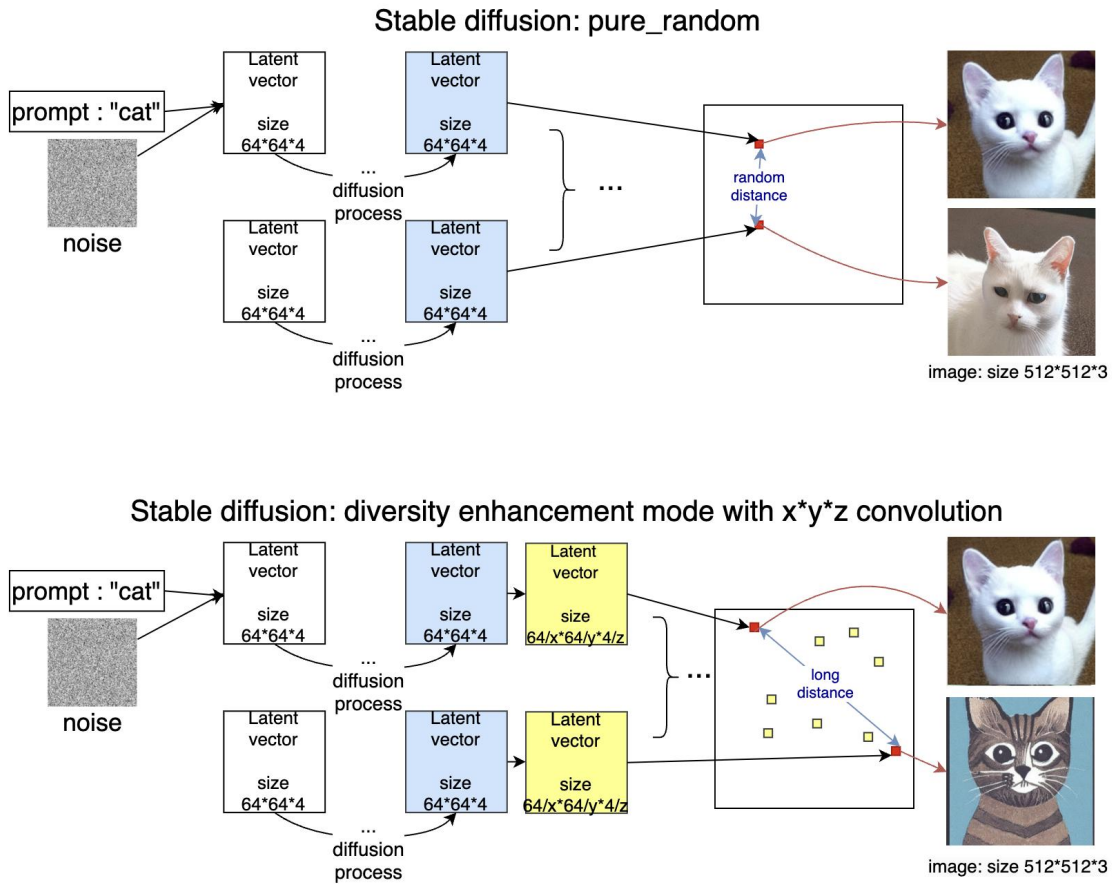
Figure 13. Top: LDM1, the pure random case.
