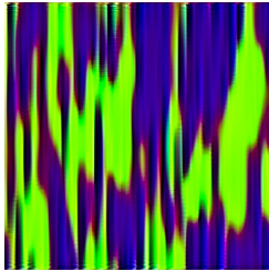
Figure 4. Example of image obtained by LDM1 with points obtained by gradient-based methods, even after standardizing the norm: images do not make any sense.
