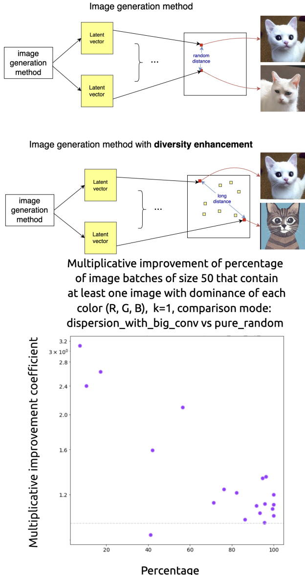
Figure 1. Top: General schema for diversity enhancement. A vanilla image generation method is compared to a method with enhanced diversity. Instead of being randomly generated, latent vectors are chosen on the basis of their pairwise distance, which results in better image diversity. Bottom: Comparison of dispersion-with-big-conv and standard LDM1 (pure-random) for various prompts: the presented numbers are the multiplicative improvement of the percentage of batches containing images with at least 2 different dominant colors for the following parameters: K = 1 , batch size = 50. In general, we get better improvement for least represented groups.
