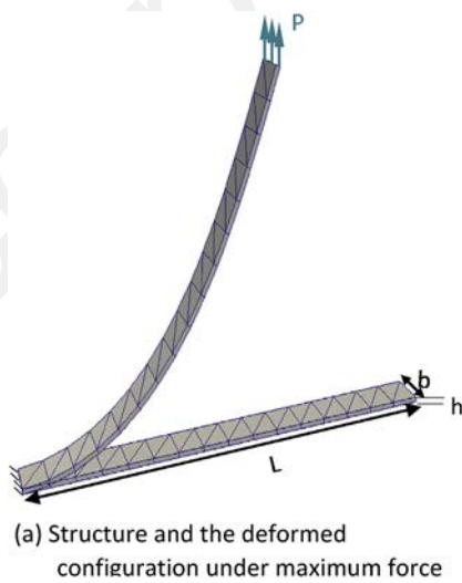
Fig. 19. Cantilever beam.
