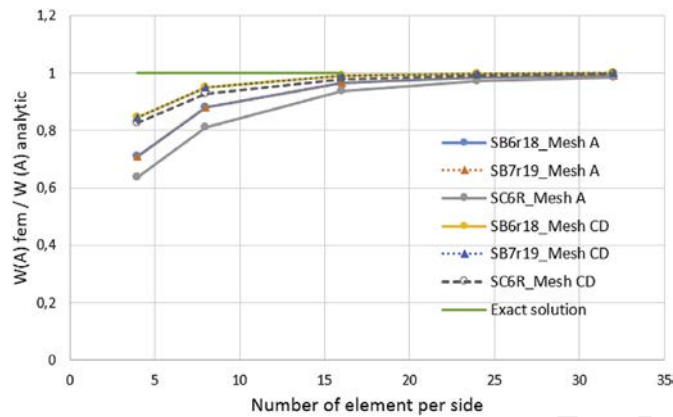
Fig. 15. Convergence of normalized deflection at free edge's mid-point w .
