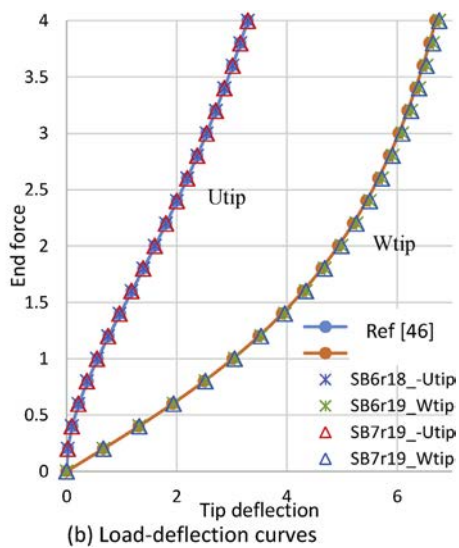
Fig. 19. Cantilever beam.
