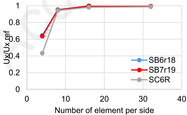
(a) Displacement of loading point
