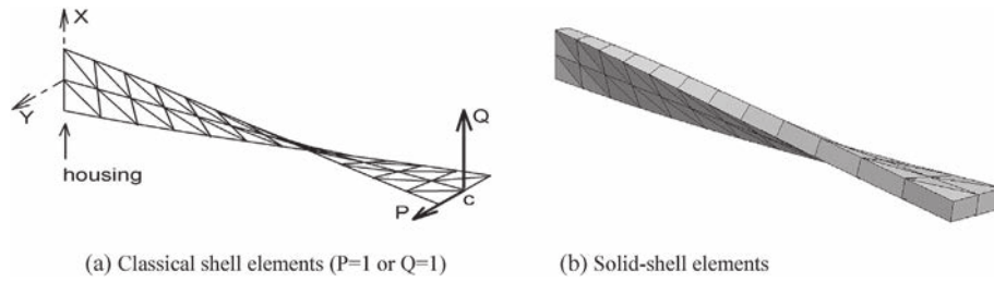
Fig. 10. Twisted beam.
