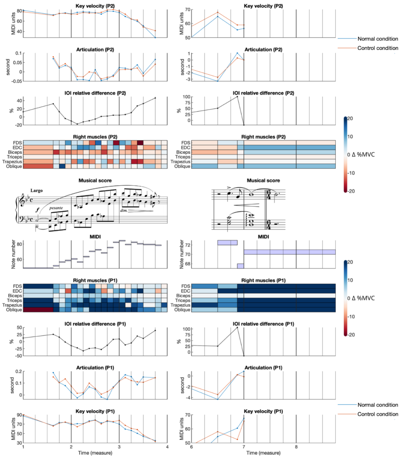
Figure 5. EMG and concrete performance features results for two passages of EI (Chopin's Ballade n. 1 op. 23) measures 1–3 (left) and measures 6–8 (right) for P1 (bottom) and P2 (top). EMG data are expressed as percentage of voluntary contraction (%MVC) and represent the difference between conditions (blue gradient being EMG activation levels higher in normal than in control condition, while red gradient being EMG activation levels higher in control than in normal condition). FDS = flexor digitorum superficialis, EDC = extensor digitorum communis, Trapezius = upper trapezius, and Oblique = external oblique. Positive articulation value = legato , negative articulation value = detaché .
