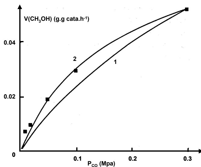
Figure 8: experimental ( \blacksquare ) rates of methanol formation as a function of P_{CO} . Curve 1 computed assuming a non-competitive adsorption between CO and H_2 , curve 2 computed assuming a competitive adsorption.
