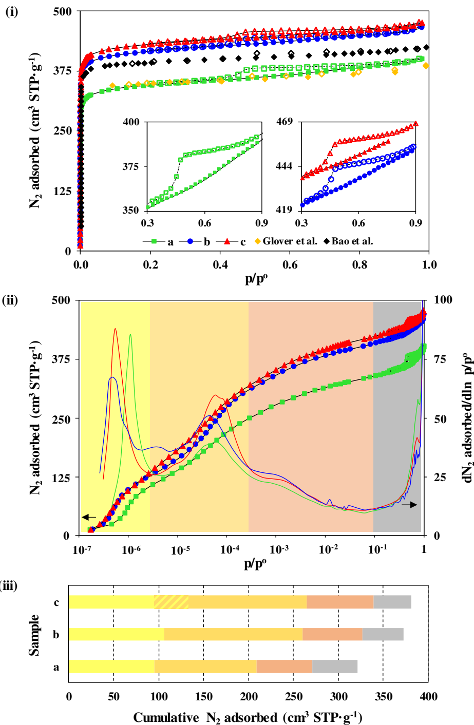
1 2 Figure 5. (i) N 2 ads/desorption isotherms at 77 K, (ii) their derivatives and (iii) cumulative N 2 3 adsorbed volume of (a) Mg-MOF-74, (b) Mg-MOF-74@CNT and (c) Mg-MOF-74@GO. 4 Solid and open symbols represent the adsorption and desorption of N 2 , respectively. 5
