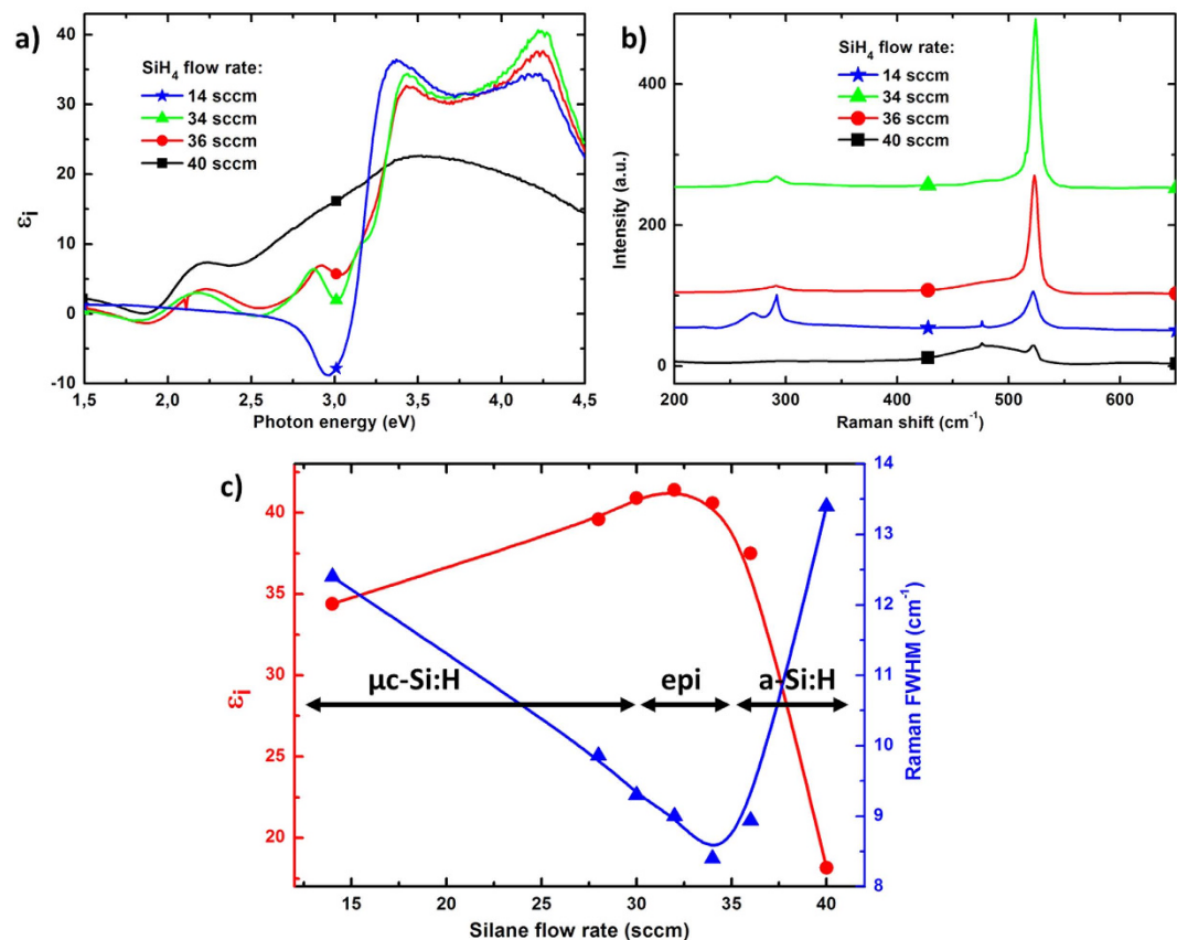
Figure 2. (a) Pseudo-dielectric function \epsilon_i of PECVD silicon layers deposited from \text{SiH}_4/\text{H}_2 on plasma cleaned GaAs wafers with various silane flow rate: 14 sccm (stars), 34 sccm (triangles), 36 sccm (circles) and 40 sccm (squares). (b) Corresponding Raman spectra. (c) Left \epsilon_i at 4.2 eV (circles) as a function of the silane flow rate. Right: FWHM of the Raman c-Si peak FWHM as a function of silane flow rate (triangles).
