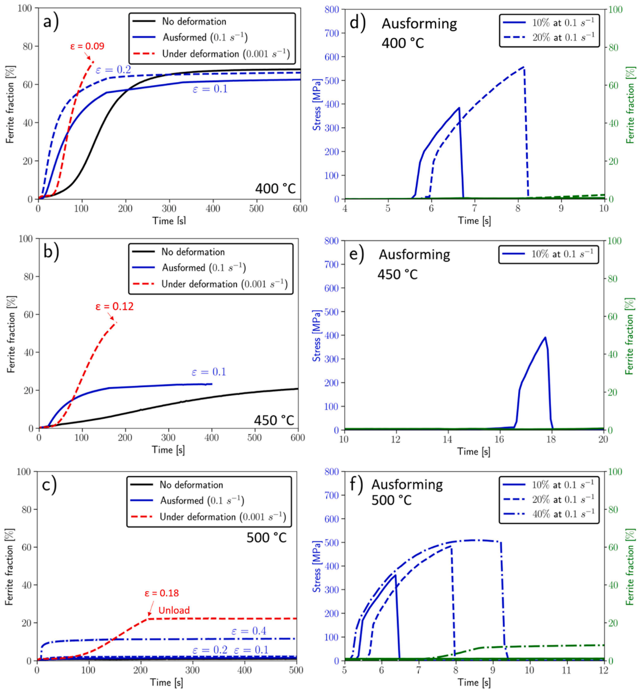
Fig. 3. : a), b) and c) HEXRD measurement of bainitic ferrite fraction evolution during thermo-mechanical processing under various deformation scenarios at different temperatures: a) 400 °C, b) 450 °C, and c) 500 °C. Deformation-free transformation is represented using black lines, ausforming using blue lines, and transformation under deformation using red lines. Figures d), e) and f) show the corresponding stress-strain curves for the ausforming process and the evolution of the ferrite fraction during ausforming step for the corresponding temperatures. The red arrows show the final strain at the end of deformation. No strain was applied beyond this point and the sample was completely unloaded.
