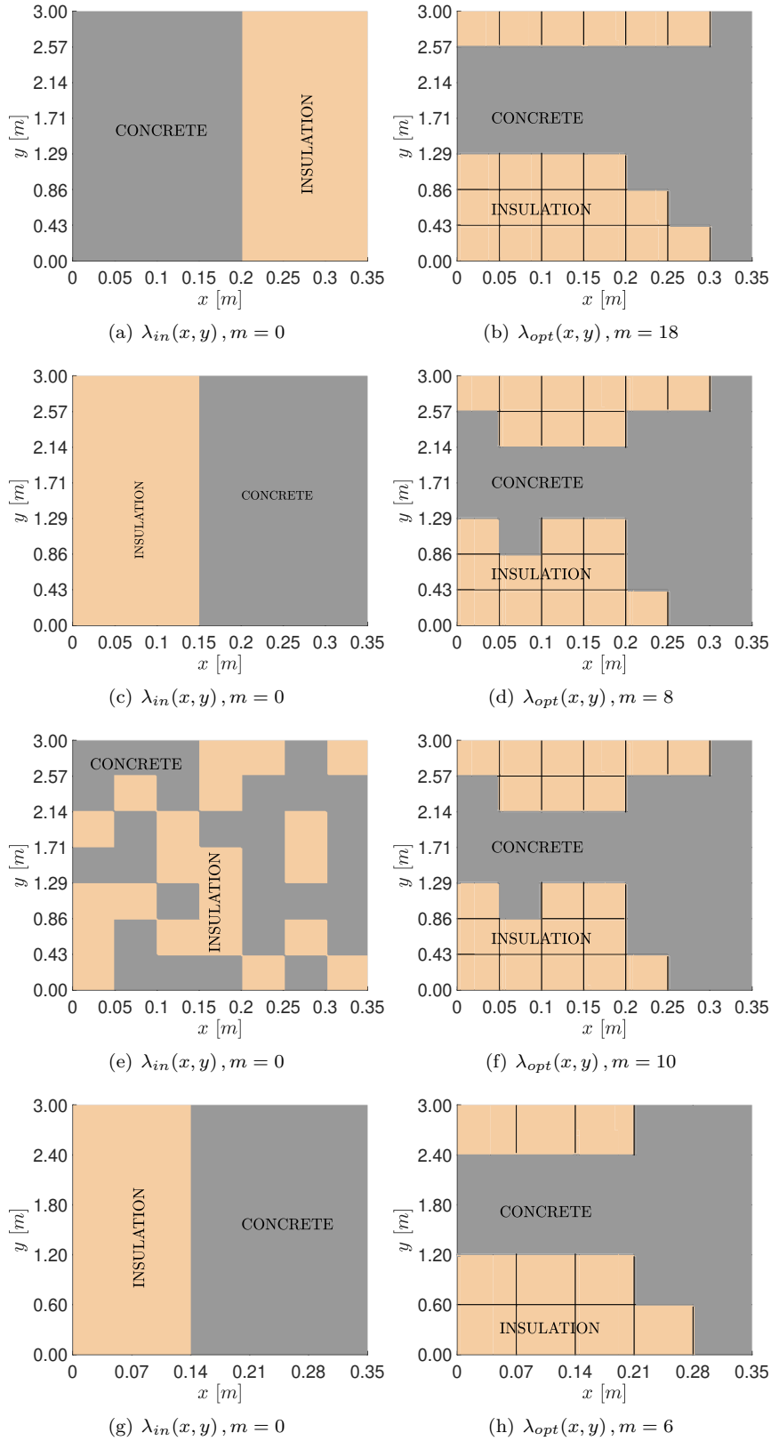
Figure 4. Design of the initial (a,c,e,g) and optimized configurations (b,d,f,h) starting with ITI distribution (a,b), ETI distribution (c,d,g,h), random distribution (e,f). Number of elementary volume is N = 49 (a-f), and N = 25 (g,h).
