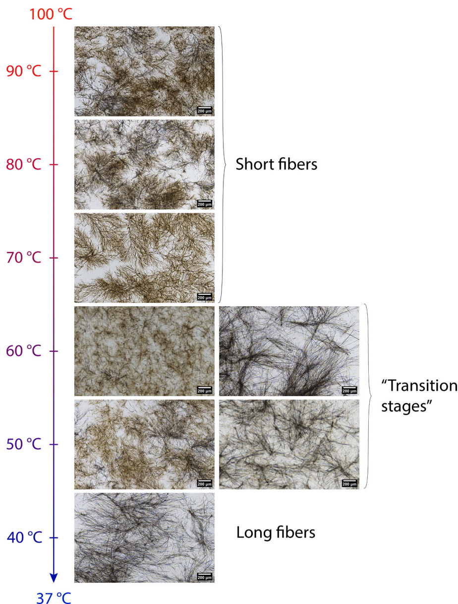
Fig. 3. Optical microscopy images showing the fiber aspect when the composite gels are taken out of the oven at different temperatures of the ramp (scale bar: 200 \mu\text{m} ).
