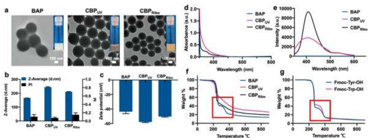
Figure 2. (a) TEM images and photographs of the solutions of the nanoparticles before and after crosslinking. (b) Size and PI assessed by DLS, and (c) surface charge (zeta potential) of the nanoparticles. (d) UV-Vis absorption spectra, and (e) fluorescence spectra of the nanoparticles (excited at 330 nm). (f) TGA of the nanoparticles before and after crosslinking. (g) TGA of the single Fmoc-amino acids.
