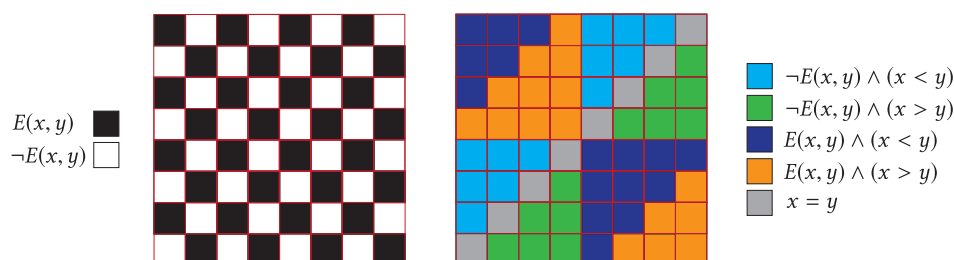
■ Figure 5 Left : The adjacency matrix of the ordered graph G with vertices 1, \dots, n and edges ij such that i + j is odd, along the usual order. (The first row is at the bottom.) Right : The adjacency matrix along another order, encoding the adjacency as well as the original order. Every 4-division contains some constant zone.
