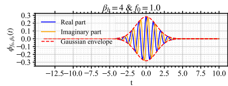
Figure 11: Complex Morlet wavelet function illustration.
