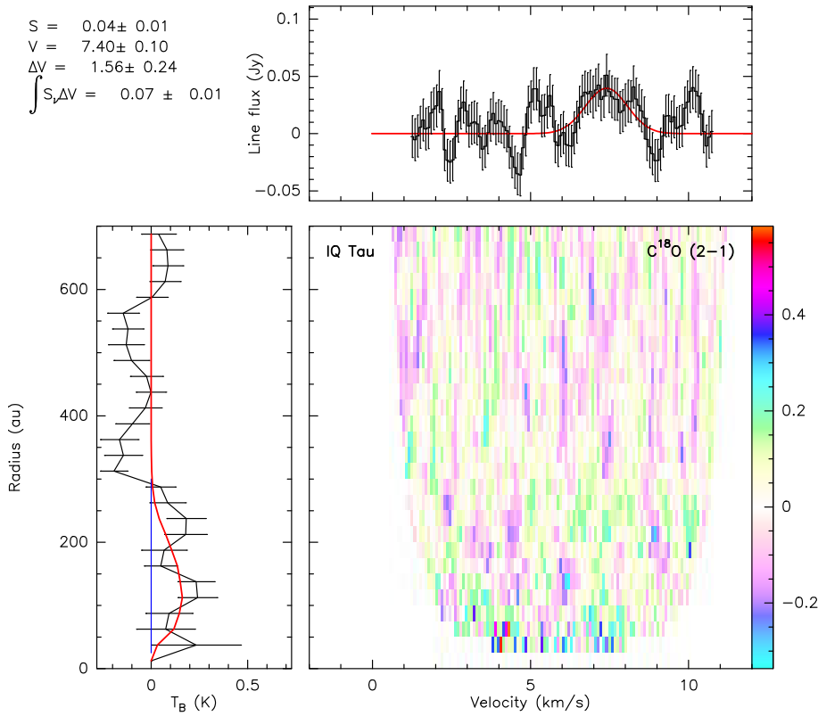
Fig. C.37. Observations of \text{C}^{18}\text{O} (2-1) emission in the IQ Tau disk. Shown is a pixel-deprojected Keplerian plot consisting of the three panels: (left) the radial profile of the line brightness temperature (K), with observations and errorbars in black, and profile derived from the best-fit disk model in red, (top) the integrated spectrum (black line) overlaid with the best-fit Gaussian profile (red line), and (bottom right) aligned and stacked line intensity (K) as a function of disk radius (Y-axis; au) and velocity (X-axis; \text{km s}^{-1} ). The color bar units are in Kelvin.
