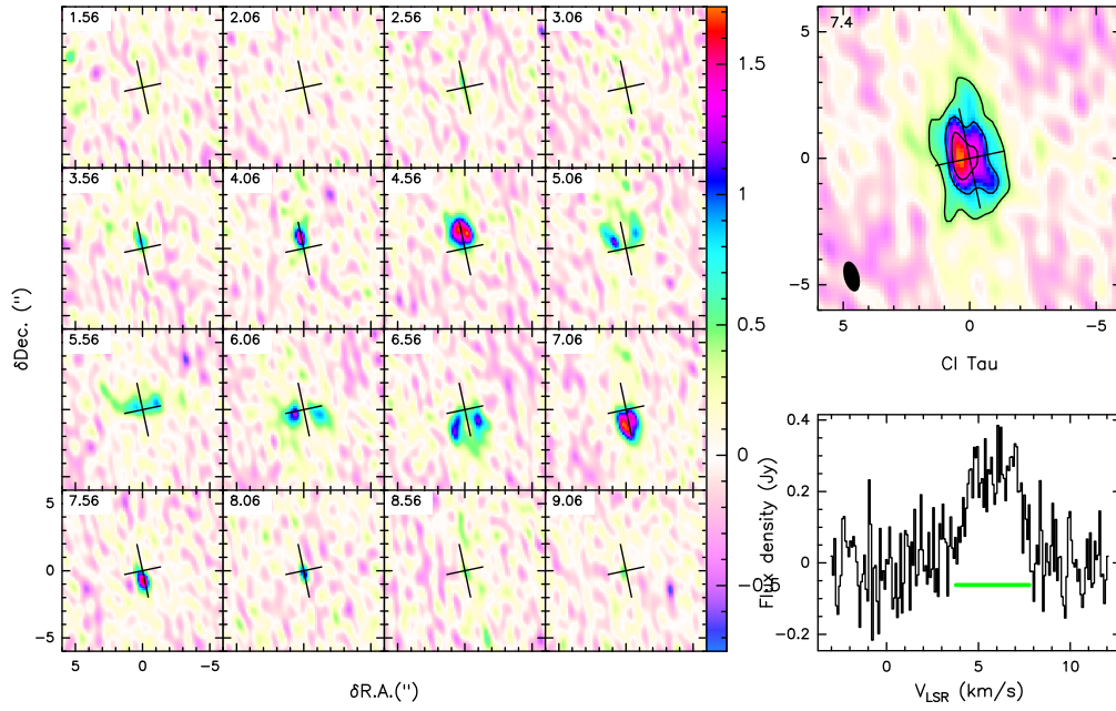
Fig. C.5. Same as Fig. C.1 but for \text{C}^{18}\text{O} (2-1) emission.
