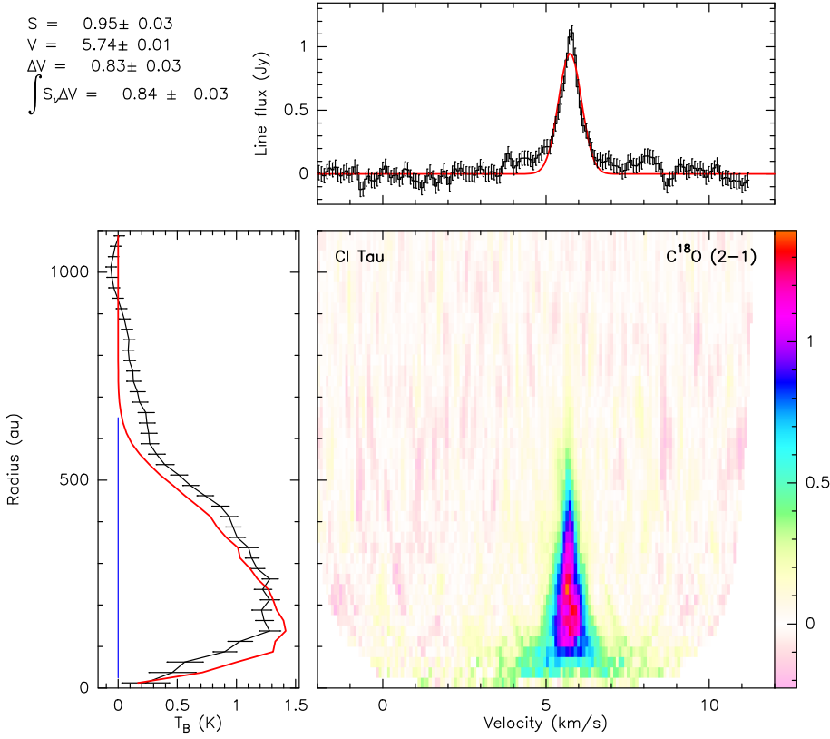
Fig. C.5. Same as Fig. C.1 but for \text{C}^{18}\text{O} (2-1) emission.
