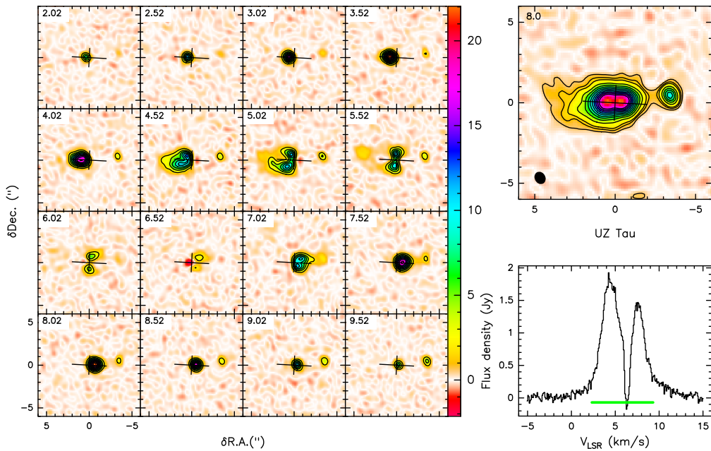
Fig. C.38. Observations of ^{12}\text{CO} (2-1) emission in the UZ Tau E disk. Shown are the channel map of the observed line brightness distribution (left), the moment-zero map (top right), and the integrated spectrum (bottom right). The channel map shows 16 velocity channels with a step of 0.5 \text{ km s}^{-1} in the [-4.5, +4.5] \text{ km s}^{-1} range around the systemic velocity. The contour lines start at 2 K, with a step of 2 K. The color bar shows line brightness temperatures (K). The contour lines in the moment-zero plot start at 3, 6, and 9\sigma , with a step of 6\sigma afterward. The 1\sigma rms noise ( \text{mJy km s}^{-1} ) is shown in the upper left corner of the moment-zero plot, and the synthesized beam is depicted by the dark ellipse in the left bottom corner.
