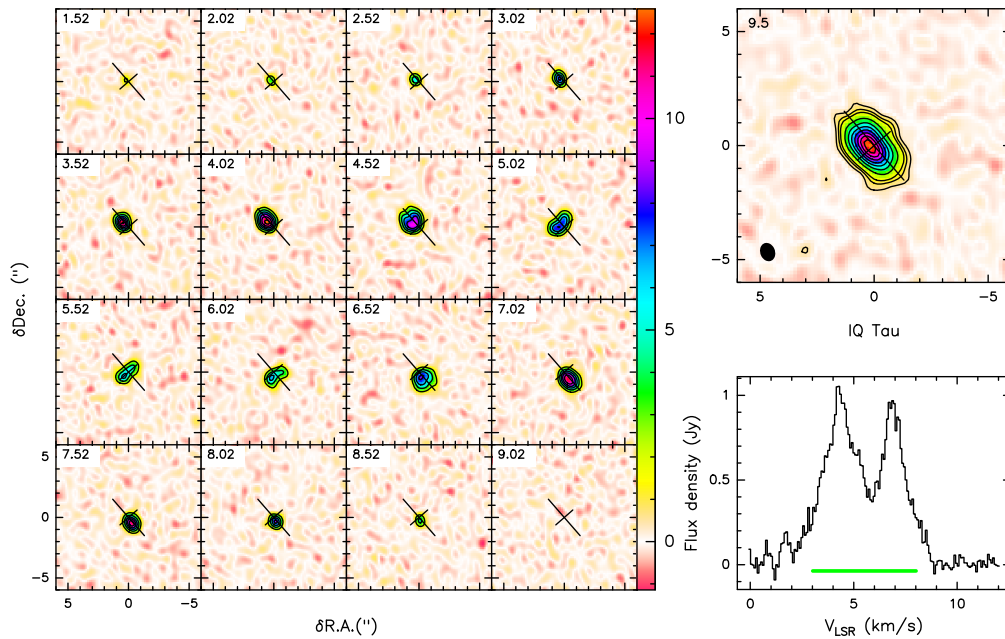
Fig. C.32. Observations of ^{12}\text{CO} (2-1) emission in the IQ Tau disk. Shown are the channel map of the observed line brightness distribution (left), the moment-zero map (top right), and the integrated spectrum (bottom right). The channel map shows 16 velocity channels with a step of 0.5 \text{ km s}^{-1} in the [-4.5, +4.5] \text{ km s}^{-1} range around the systemic velocity. The contour lines start at 2 K, with a step of 2 K. The color bar shows line brightness temperatures (K). The contour lines in the moment-zero plot start at 3, 6, and 9\sigma , with a step of 6\sigma afterward. The 1\sigma rms noise ( \text{mJy km s}^{-1} ) is shown in the upper left corner of the moment-zero plot, and the synthesized beam is depicted by the dark ellipse in the left bottom corner.
