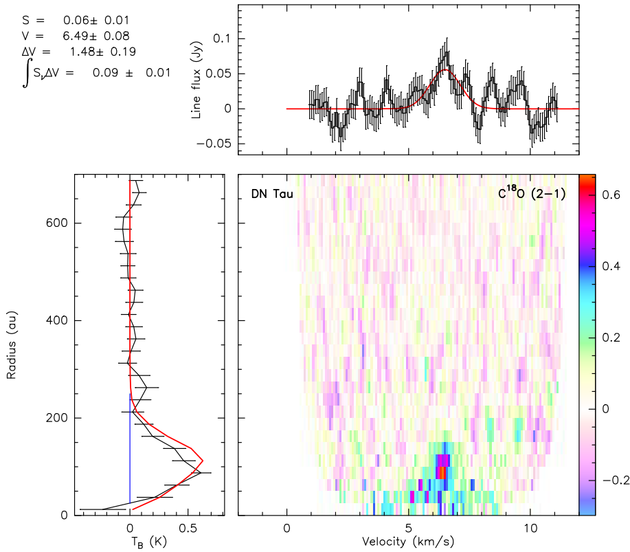
Fig. C.31. Observations of \text{C}^{18}\text{O} (2-1) emission in the DN Tau disk. Shown is a pixel-deprojected Keplarian plot consisting of the three panels: (left) the radial profile of the line brightness temperature (K), with observations and errorbars in black, and profile derived from the best-fit disk model in red, (top) the integrated spectrum (black line) overlaid with the best-fit Gaussian profile (red line), and (bottom right) aligned and stacked line intensity (K) as a function of disk radius (Y-axis; au) and velocity (X-axis; \text{km s}^{-1} ). The color bar units are in Kelvin.
