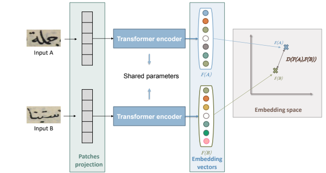
Fig. 1. The method involves mapping two input word images into a common feature space via the use of transformers and utilizing a contrastive loss function to train the model. The Siamese transformer architectures allow the model to learn the similarities and differences between the two input word images, enabling it to effectively identify and match word images in the common feature space.
