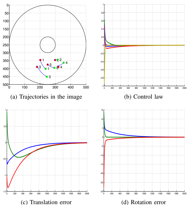
Fig. 3. Simulation: Positioning an omni-directional camera with a parabolic mirror with respect to an unknown planar target without using any approximation on its 3D parameters.
