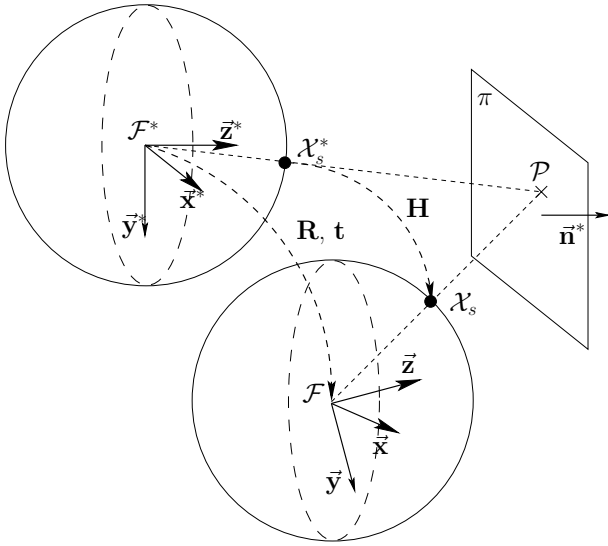
Fig. 2. Homography from two spherical projections.
