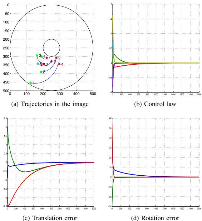
Fig. 4. Simulation: Positioning an omni-directional camera with a hyperbolic mirror with respect to an unknown planar target without using any approximation on its 3D parameters.
