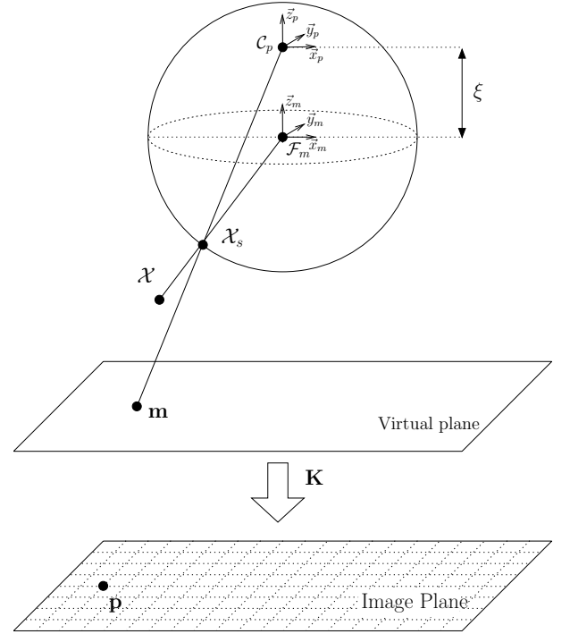
Fig. 1. Projection model for central catadioptric cameras
