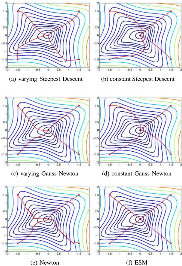
Fig. 1. Comparing the behavior of 6 different minimization methods.
