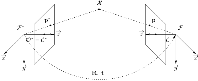
Figure 1: Perspective projection of a point. The parameters involved in the projection are roughly known.
