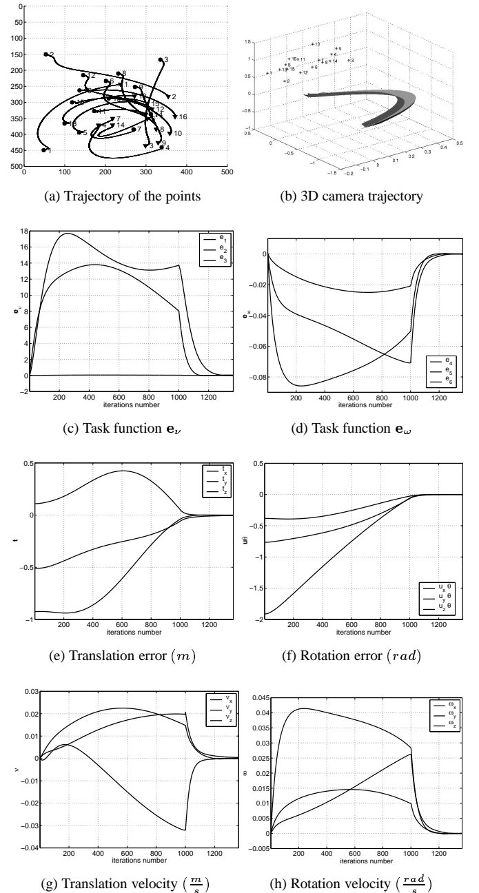
Figure 4: Simulation with large calibration errors, with the same initial displacement but with path planning.
