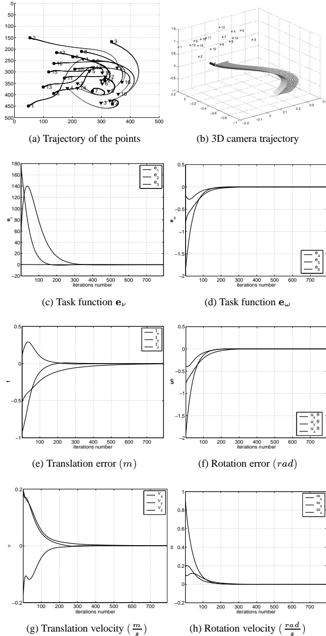
Figure 3: Simulation with large calibration errors and large initial displacement of the end-effector of the robot.
