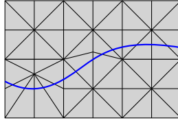
(b) The perturbed triangulation L^* , which is in general position with respect to \iota(\mathcal{M}) .
