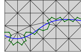
(c) The resulting triangulation \mathcal{T} of \mathcal{M} (dark green). \mathcal{T} is a subcomplex of (L^*)' .
