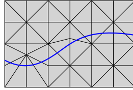
(b) The perturbed triangulation L^* , which is in general position with respect to \iota(\mathcal{M}) .
