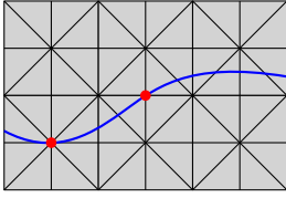
(a) The triangulation L and the image \iota(\mathcal{M}) (blue). The red points indicate the vertices of L contained by \iota(\mathcal{M}) .
