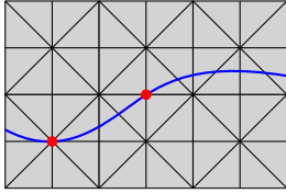
(a) The triangulation L and the image \iota(\mathcal{M}) (blue). The red points indicate the vertices of L contained by \iota(\mathcal{M}) .
