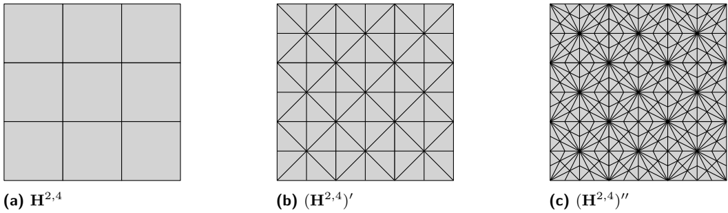
■ Figure 5 The effect of two barycentric subdivisions on the 2-dimensional hypercubic honeycomb.
