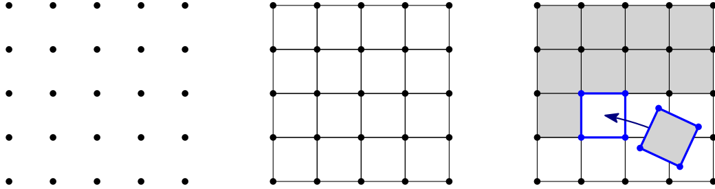
■ Figure 2 Constructing the complex \mathbf{H}^{2,5} . Its 1-skeleton \mathbf{H}_1^{2,5} is isomorphic to the grid P_5^2 .
