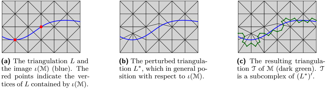
■ Figure 6 Illustration of Whitney’s method of triangulating ambient submanifolds ( d = 1 ).
