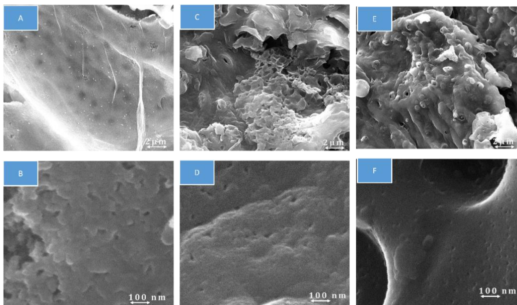
Figure 5: SEM images of samples (A) PPAC_WS_N2_1173 (Scale bar = 2 \mu\text{m} ); (B) PPAC_WS_N2_1173 (Scale bar = 100 nm); (C) PPAC_PEL_N2_1173 (Scale bar = 2 \mu\text{m} ); (D) PPAC_PEL_N2_1173 (Scale bar = 100 nm); (E) PPAC_POW_N2_1173 (Scale bar = 2 \mu\text{m} ); (F) PPAC_POW_N2_1173 (Scale bar = 100 nm).
