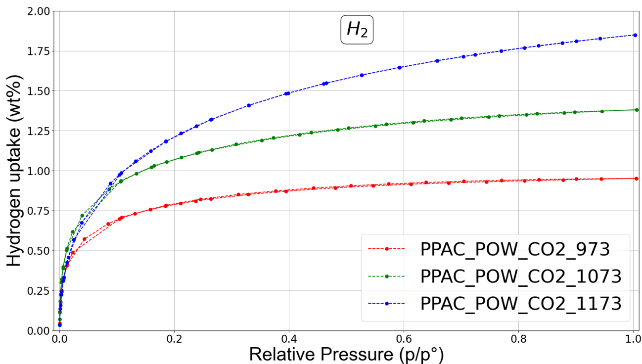
Figure 12: H_2 adsorption isotherms of samples PPAC_POW_CO2_973, PPAC_POW_CO2_1073, PPAC_POW_CO2_1173 measured at 77 K up to 1 bar.
