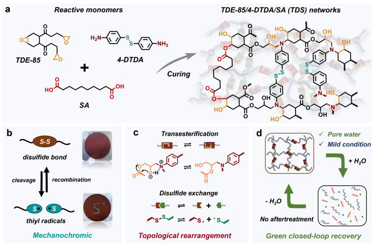
Scheme 1. Design concept of TDE-85/4-DTDA/SA (TDS) networks featuring dynamic ester and disulfide bonds. a) Chemical structures of reactive monomers and the cross-linked networks. b) Damage and healing sensing functions promoted by the reversible transformation between disulfide bonds and thiyl radicals. c) Topological network rearrangements facilitated by the harmonious interplay between disulfide and ester bonds-promoted by tertiary amine. d) Schematic illustration of the green closed-loop recovery.
