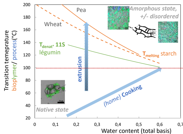
Figure 2: State diagram of legume biopolymers, with two processing paths, and micrographs (CSLM 2 , 100 \mu\text{m} , INRAE) showing the composite starch (grey) / protein (green) morphology, and scheme of denatured protein, above transition temperature. Arrows indicate two possible hydrothermal processing pathways.
