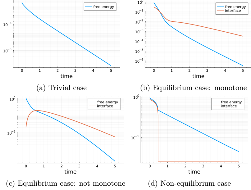
Figure 6: \mathcal{H}(\mathbf{c}^p, X^p) - \mathcal{H}(\mathbf{c}^\infty, X^\infty) and |X^\infty - X^p| for different test cases
